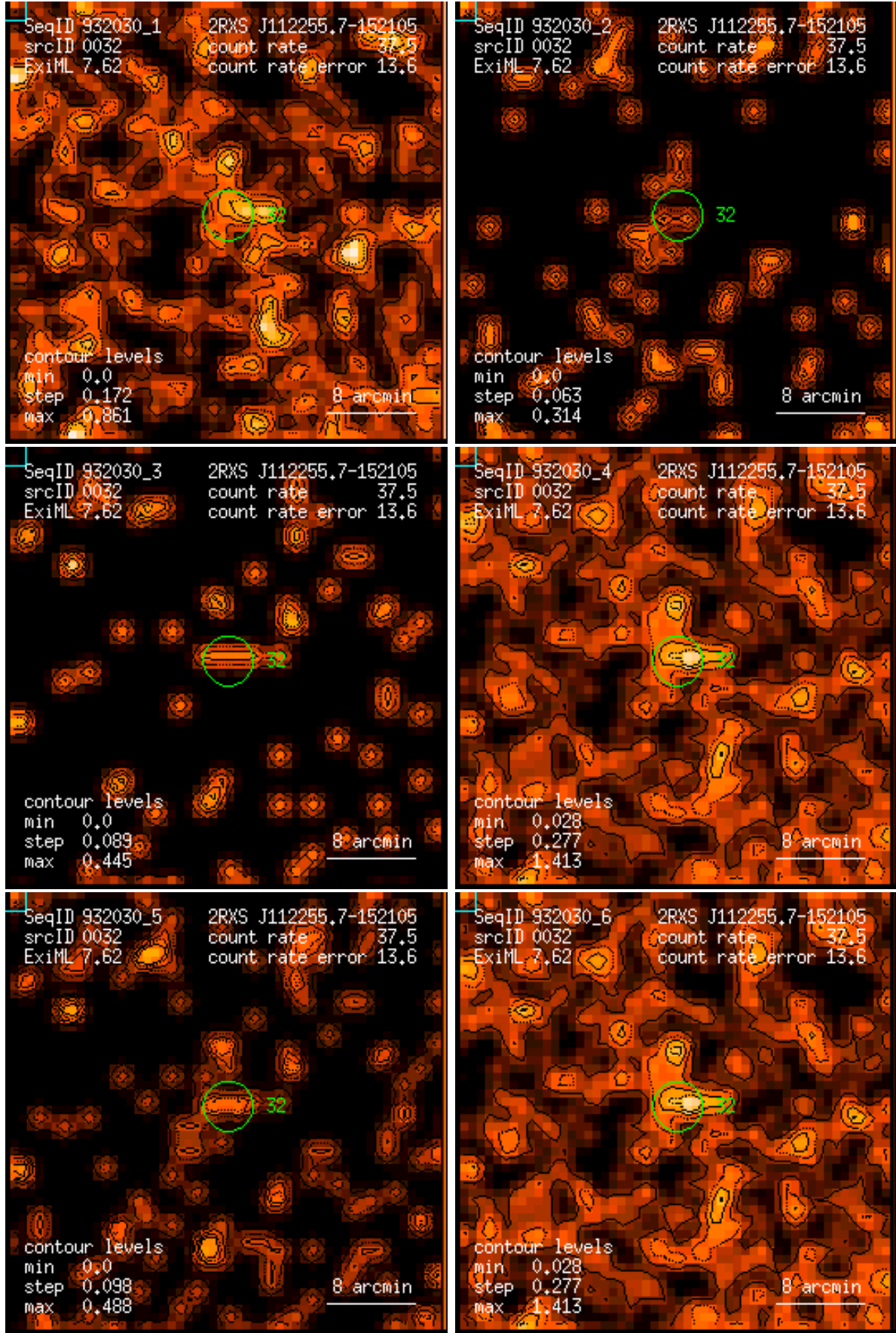
Figure 32: RASS 932030: detection 0032: band rate images, Gaussian filter: (1) PSPC channels 11 – 41, (2) 52 – 90, (3) 91 – 201, (4) 11 – 235, (5) 52 – 201, (6) 11 – 201. Broad band rates in counts/ks. Band rate contour levels in counts/ks/arcmin 2 .
