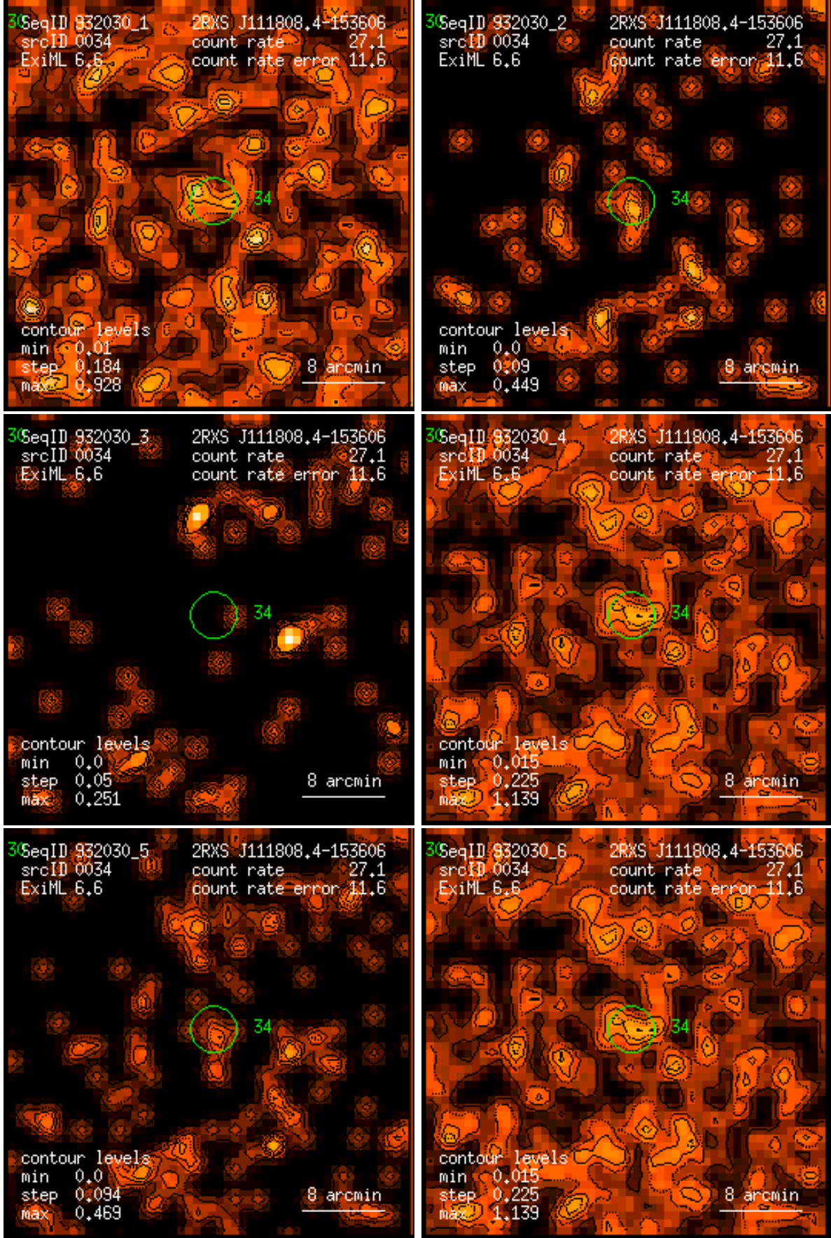
Figure 34: RASS 932030: detection 0034: band rate images, Gaussian filter: (1) PSPC channels 11 – 41, (2) 52 – 90, (3) 91 – 201, (4) 11 – 235, (5) 52 – 201, (6) 11 – 201. Broad band rates in counts/ks. Band rate contour levels in counts/ks/arcmin 2 .
