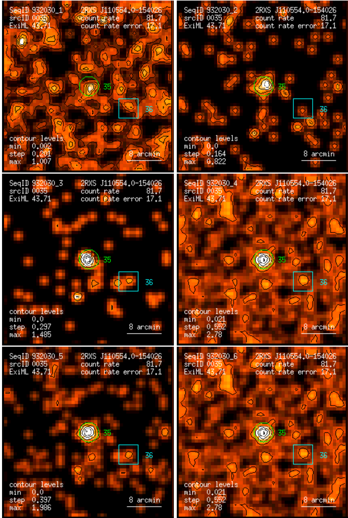
Figure 35: RASS 932030: detection 0035: band rate images, Gaussian filter: (1) PSPC channels 11 – 41, (2) 52 – 90, (3) 91 – 201, (4) 11 – 235, (5) 52 – 201, (6) 11 – 201. Broad band rates in counts/ks. Band rate contour levels in counts/ks/arcmin 2 .
