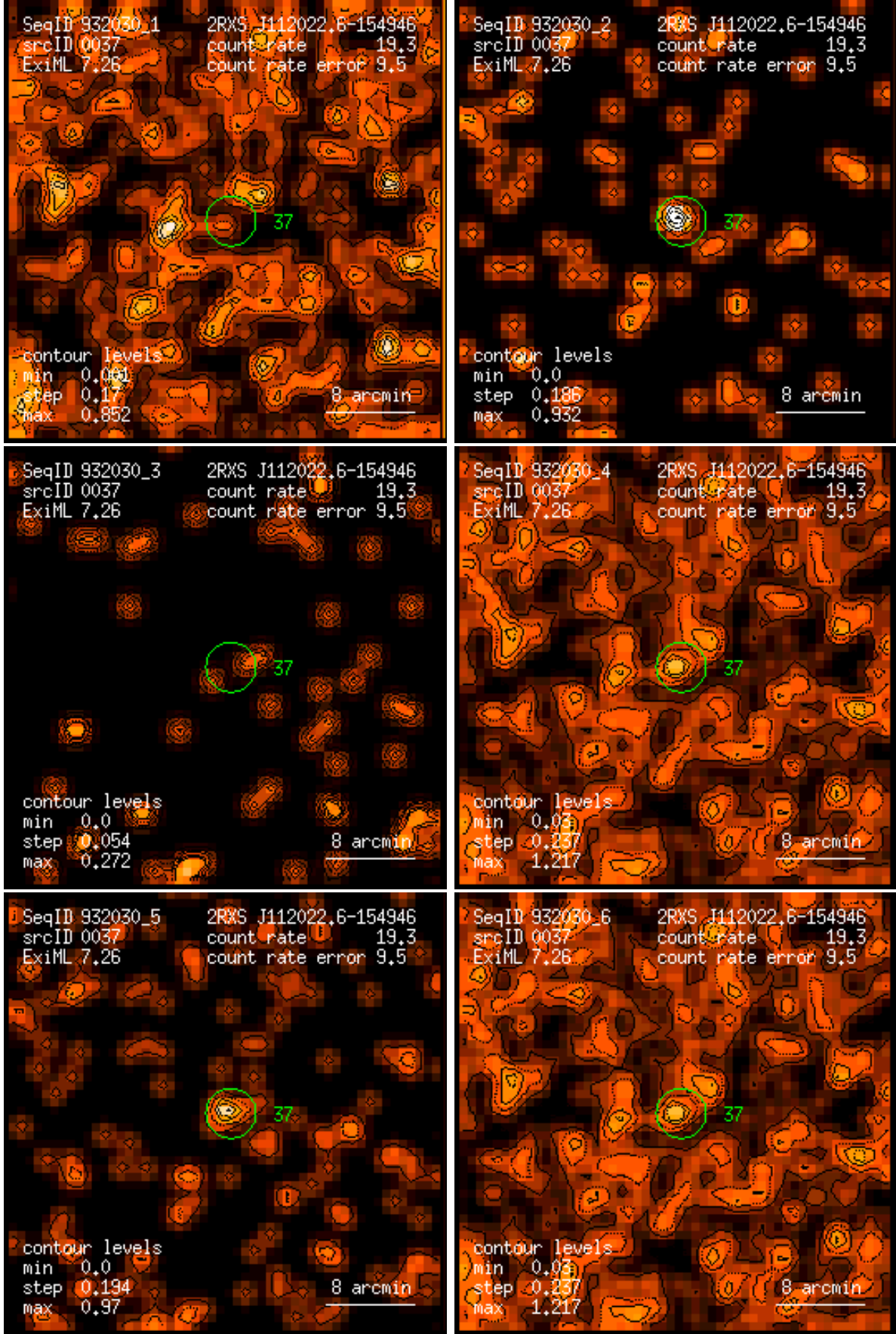
Figure 37: RASS 932030: detection 0037: band rate images, Gaussian filter: (1) PSPC channels 11 – 41, (2) 52 – 90, (3) 91 – 201, (4) 11 – 235, (5) 52 – 201, (6) 11 – 201. Broad band rates in counts/ks. Band rate contour levels in counts/ks/arcmin 2 .
