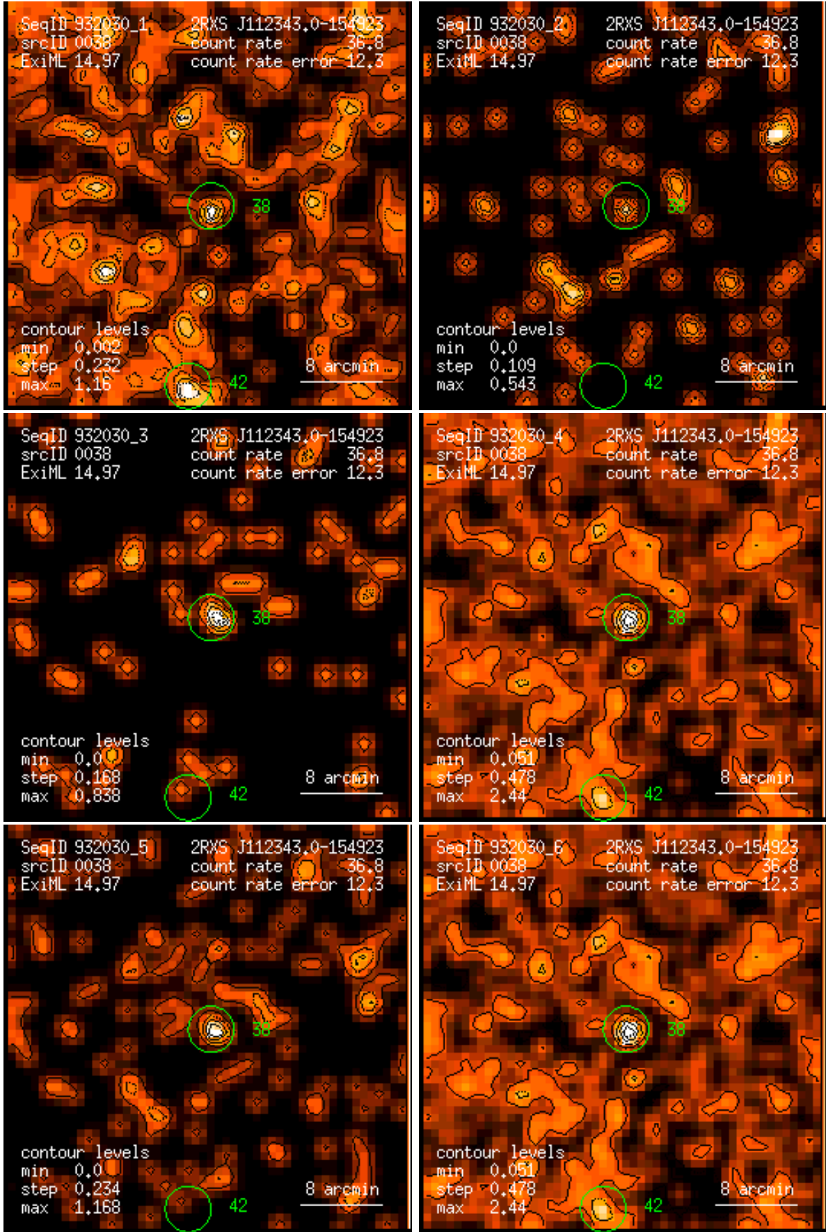
Figure 38: RASS 932030: detection 0038: band rate images, Gaussian filter: (1) PSPC channels 11 – 41, (2) 52 – 90, (3) 91 – 201, (4) 11 – 235, (5) 52 – 201, (6) 11 – 201. Broad band rates in counts/ks. Band rate contour levels in counts/ks/arcmin 2 .
