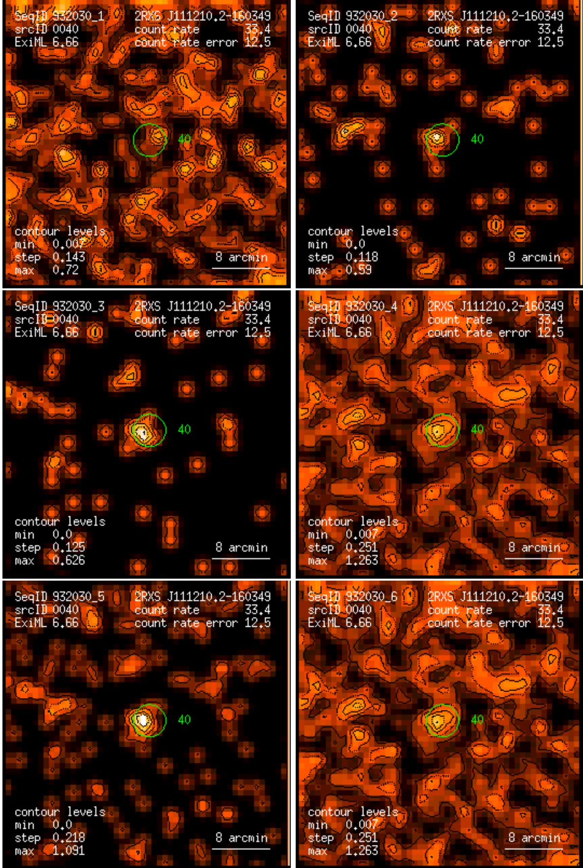
Figure 40: RASS 932030: detection 0040: band rate images, Gaussian filter: (1) PSPC channels 11 – 41, (2) 52 – 90, (3) 91 – 201, (4) 11 – 235, (5) 52 – 201, (6) 11 – 201. Broad band rates in counts/ks. Band rate contour levels in counts/ks/arcmin 2 .
