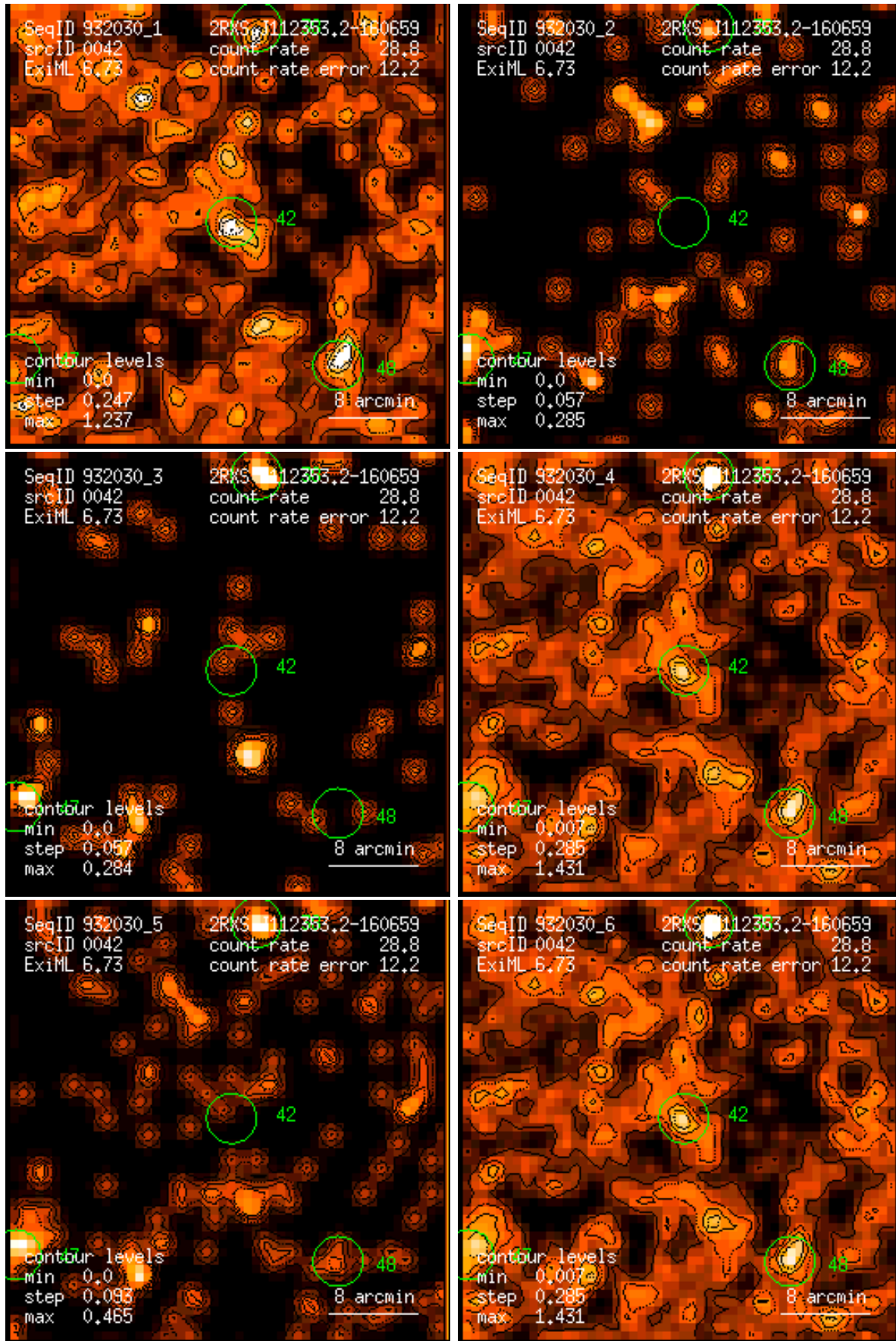
Figure 42: RASS 932030: detection 0042: band rate images, Gaussian filter: (1) PSPC channels 11 – 41, (2) 52 – 90, (3) 91 – 201, (4) 11 – 235, (5) 52 – 201, (6) 11 – 201. Broad band rates in counts/ks. Band rate contour levels in counts/ks/arcmin 2 .
