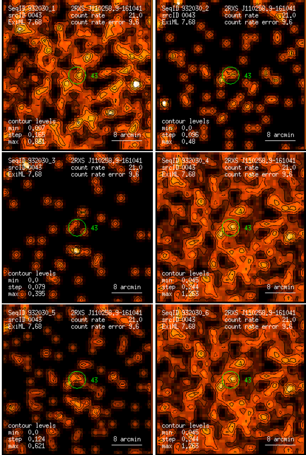
Figure 43: RASS 932030: detection 0043: band rate images, Gaussian filter: (1) PSPC channels 11 – 41, (2) 52 – 90, (3) 91 – 201, (4) 11 – 235, (5) 52 – 201, (6) 11 – 201. Broad band rates in counts/ks. Band rate contour levels in counts/ks/arcmin 2 .
