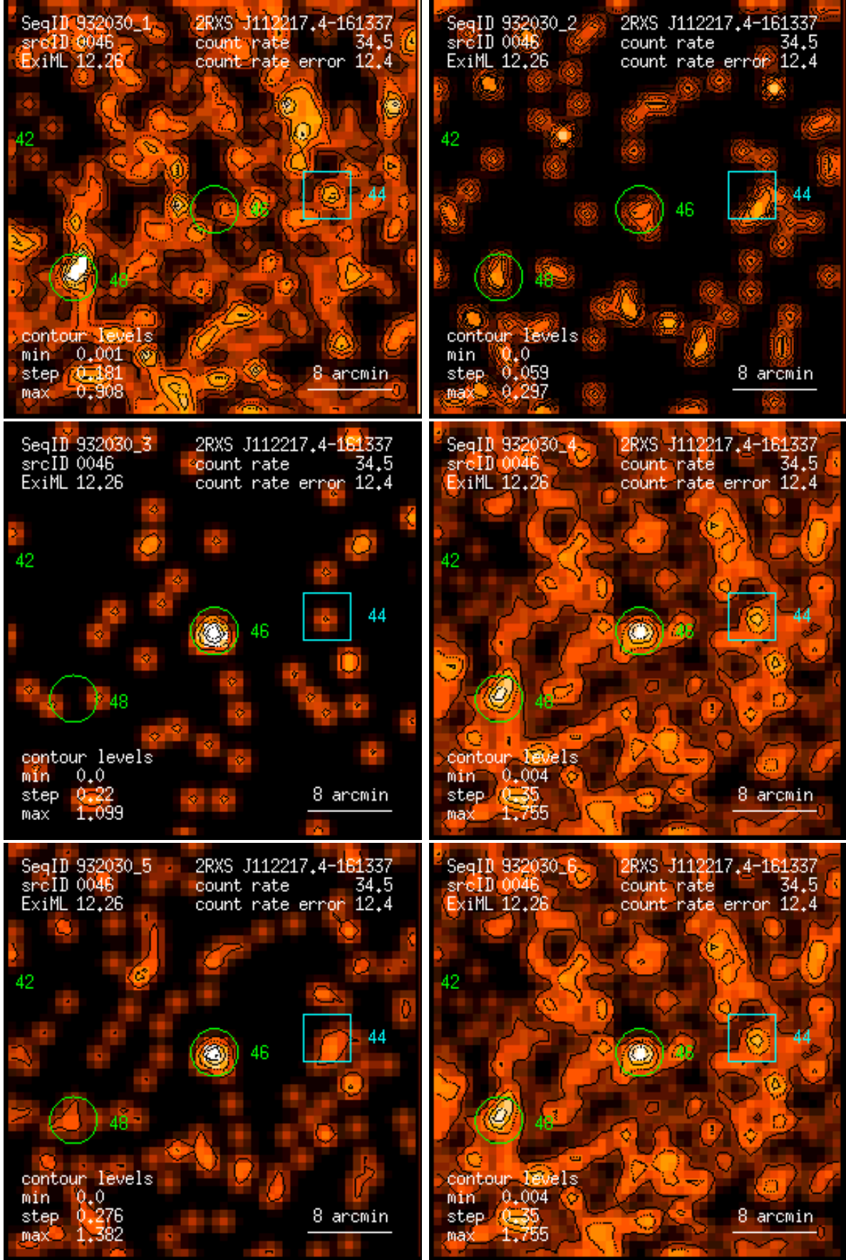
Figure 46: RASS 932030: detection 0046: band rate images, Gaussian filter: (1) PSPC channels 11 – 41, (2) 52 – 90, (3) 91 – 201, (4) 11 – 235, (5) 52 – 201, (6) 11 – 201. Broad band rates in counts/ks. Band rate contour levels in counts/ks/arcmin 2 .
