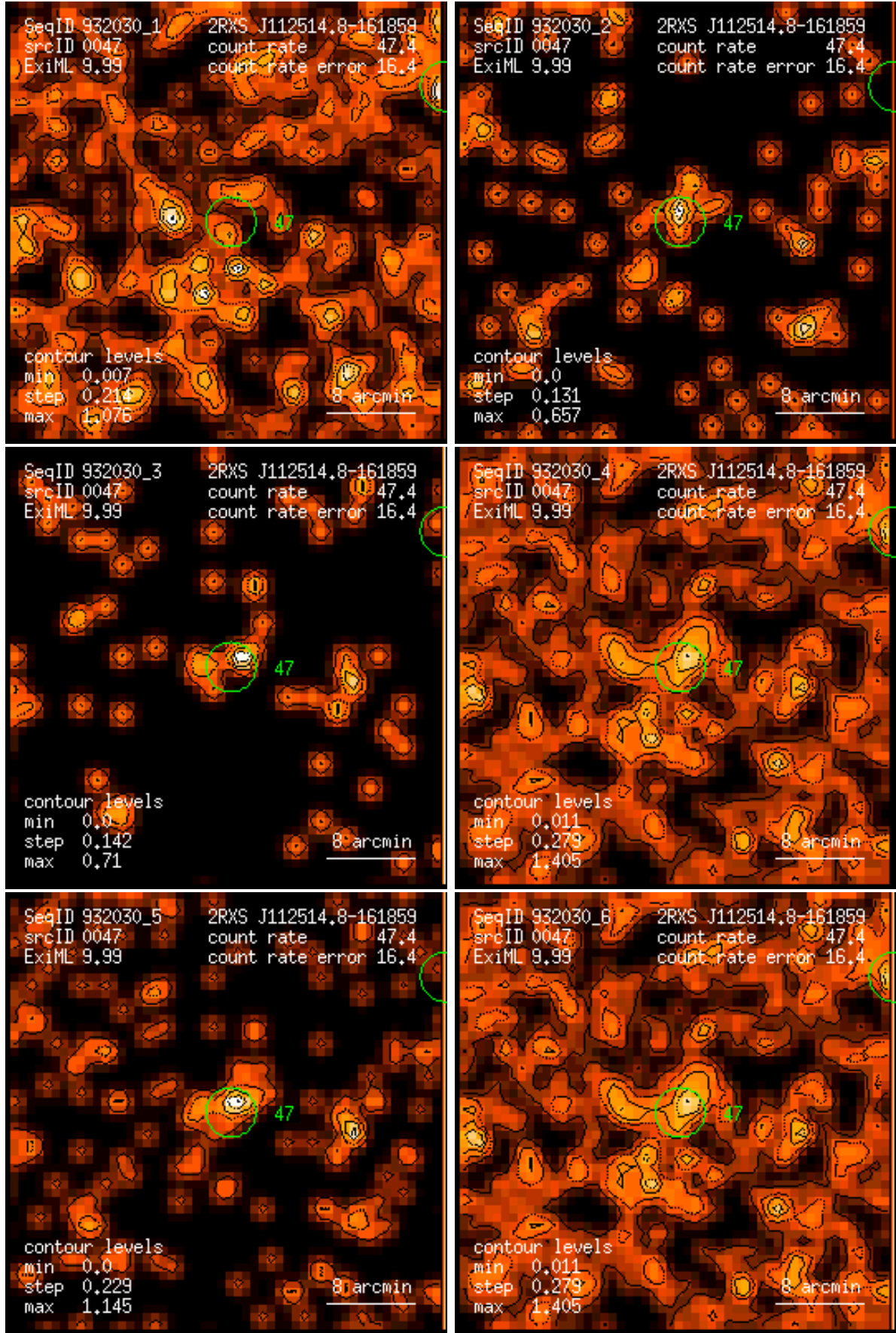
Figure 47: RASS 932030: detection 0047: band rate images, Gaussian filter: (1) PSPC channels 11 – 41, (2) 52 – 90, (3) 91 – 201, (4) 11 – 235, (5) 52 – 201, (6) 11 – 201. Broad band rates in counts/ks. Band rate contour levels in counts/ks/arcmin 2 .
