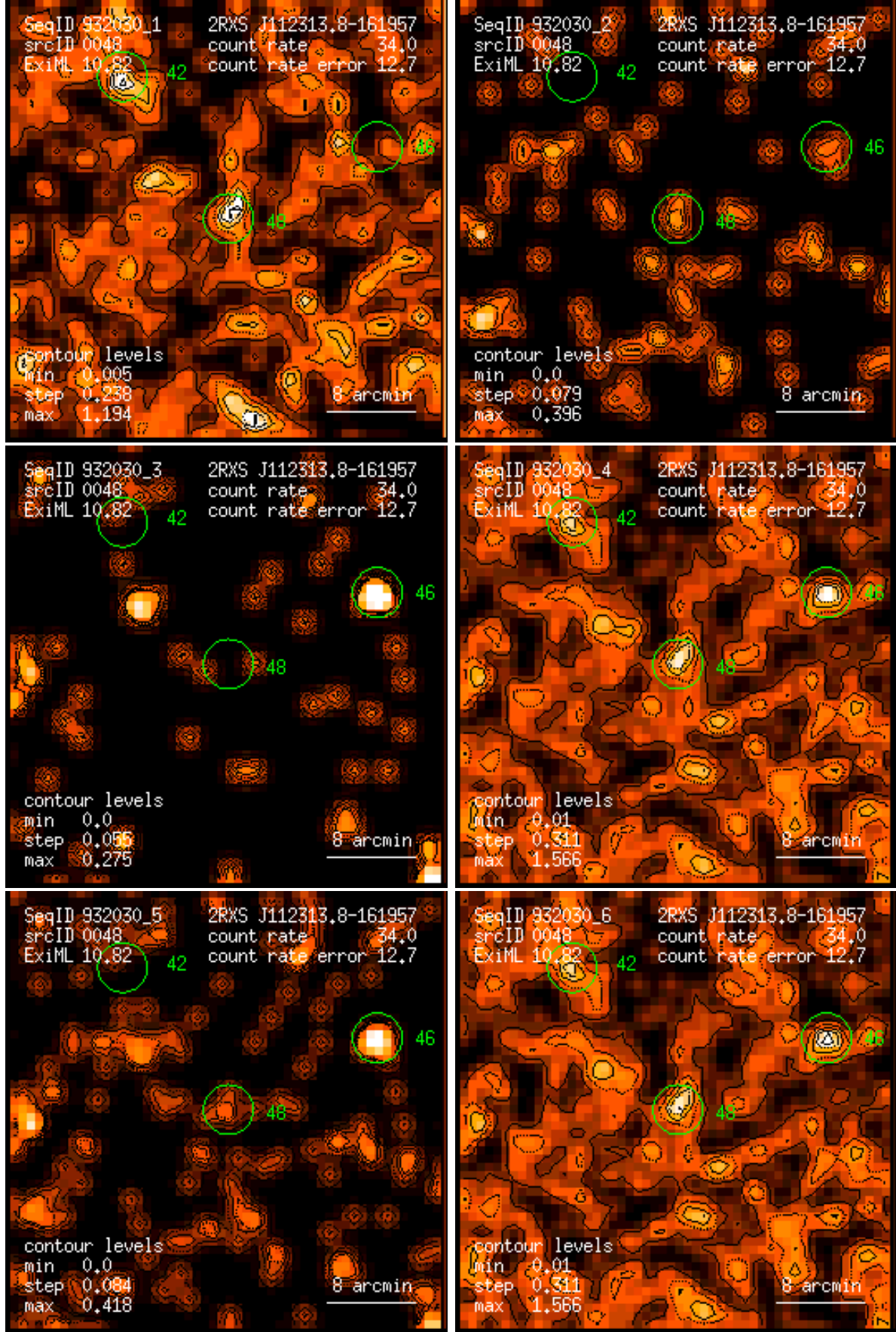
Figure 48: RASS 932030: detection 0048: band rate images, Gaussian filter: (1) PSPC channels 11 – 41, (2) 52 – 90, (3) 91 – 201, (4) 11 – 235, (5) 52 – 201, (6) 11 – 201. Broad band rates in counts/ks. Band rate contour levels in counts/ks/arcmin 2 .
