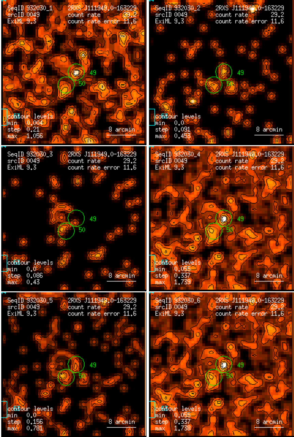
Figure 49: RASS 932030: detection 0049: band rate images, Gaussian filter: (1) PSPC channels 11 – 41, (2) 52 – 90, (3) 91 – 201, (4) 11 – 235, (5) 52 – 201, (6) 11 – 201. Broad band rates in counts/ks. Band rate contour levels in counts/ks/arcmin 2 .
