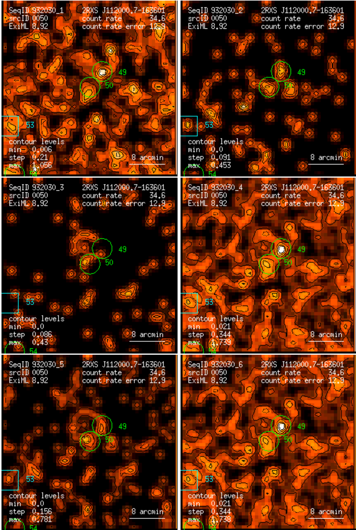
Figure 50: RASS 932030: detection 0050: band rate images, Gaussian filter: (1) PSPC channels 11 – 41, (2) 52 – 90, (3) 91 – 201, (4) 11 – 235, (5) 52 – 201, (6) 11 – 201. Broad band rates in counts/ks. Band rate contour levels in counts/ks/arcmin 2 .
