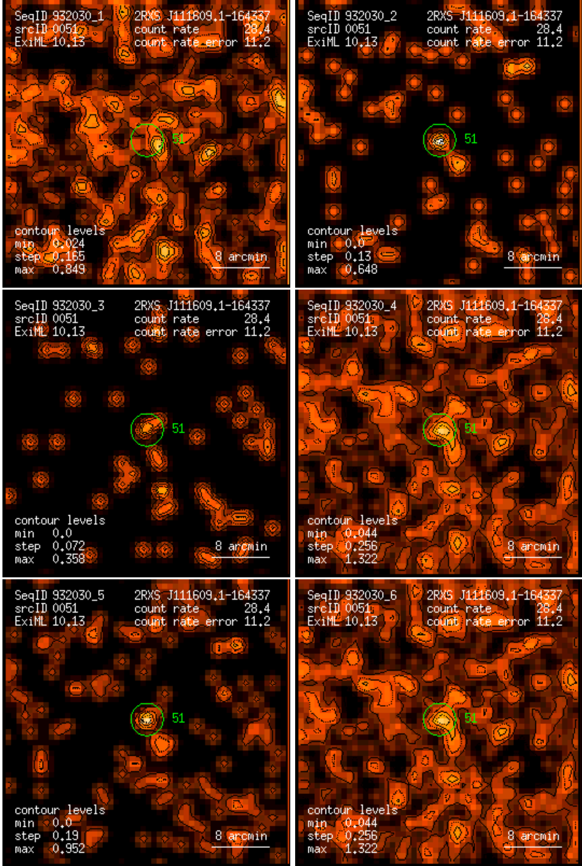
Figure 51: RASS 932030: detection 0051: band rate images, Gaussian filter: (1) PSPC channels 11 – 41, (2) 52 – 90, (3) 91 – 201, (4) 11 – 235, (5) 52 – 201, (6) 11 – 201. Broad band rates in counts/ks. Band rate contour levels in counts/ks/arcmin 2 .
