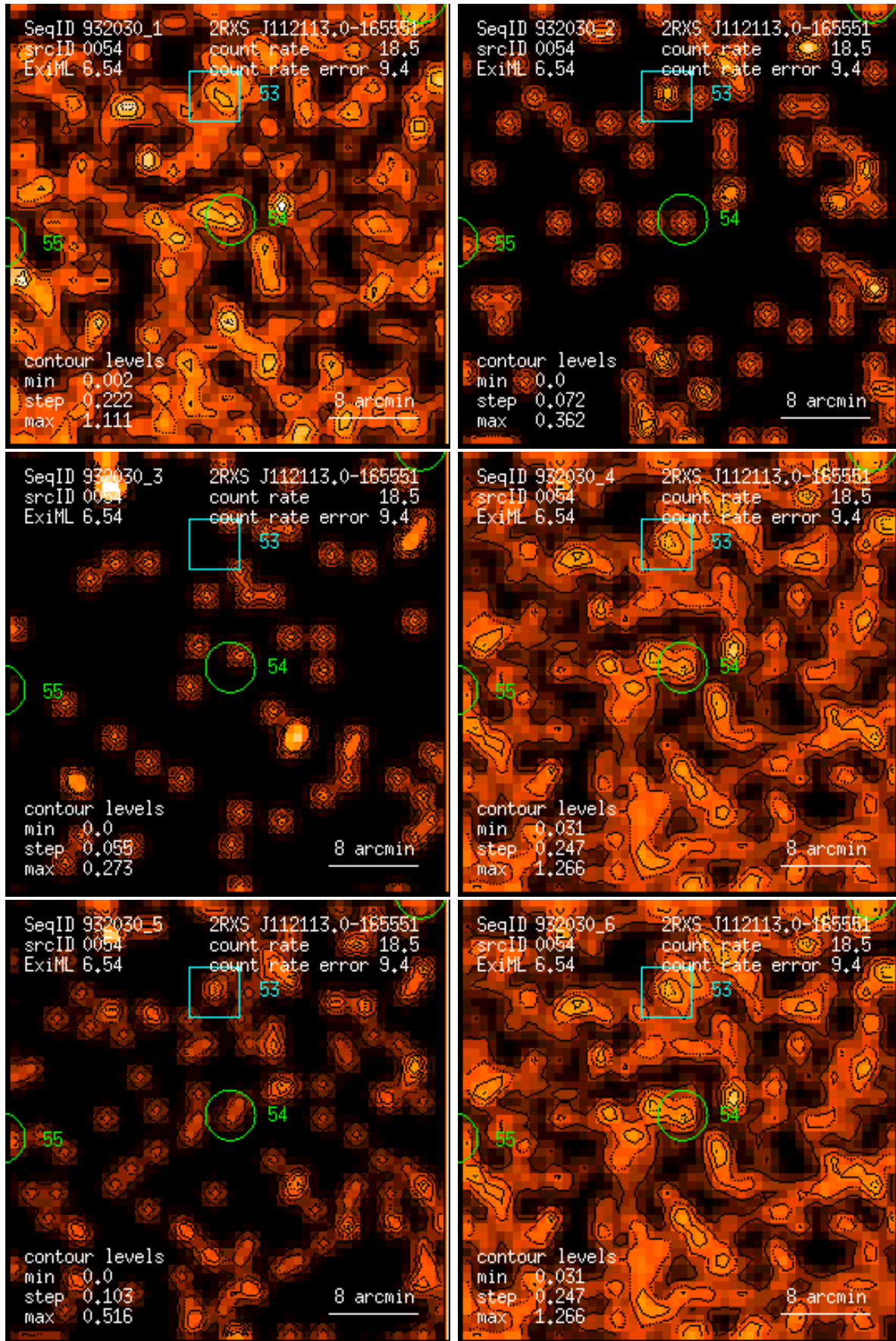
Figure 54: RASS 932030: detection 0054: band rate images, Gaussian filter: (1) PSPC channels 11 – 41, (2) 52 – 90, (3) 91 – 201, (4) 11 – 235, (5) 52 – 201, (6) 11 – 201. Broad band rates in counts/ks. Band rate contour levels in counts/ks/arcmin 2 .
