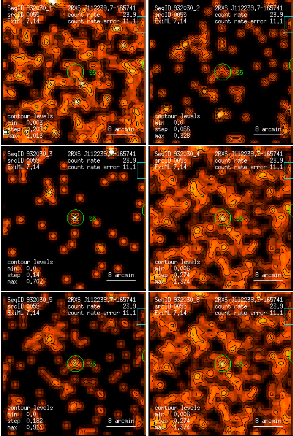
Figure 55: RASS 932030: detection 0055: band rate images, Gaussian filter: (1) PSPC channels 11 – 41, (2) 52 – 90, (3) 91 – 201, (4) 11 – 235, (5) 52 – 201, (6) 11 – 201. Broad band rates in counts/ks. Band rate contour levels in counts/ks/arcmin 2 .
