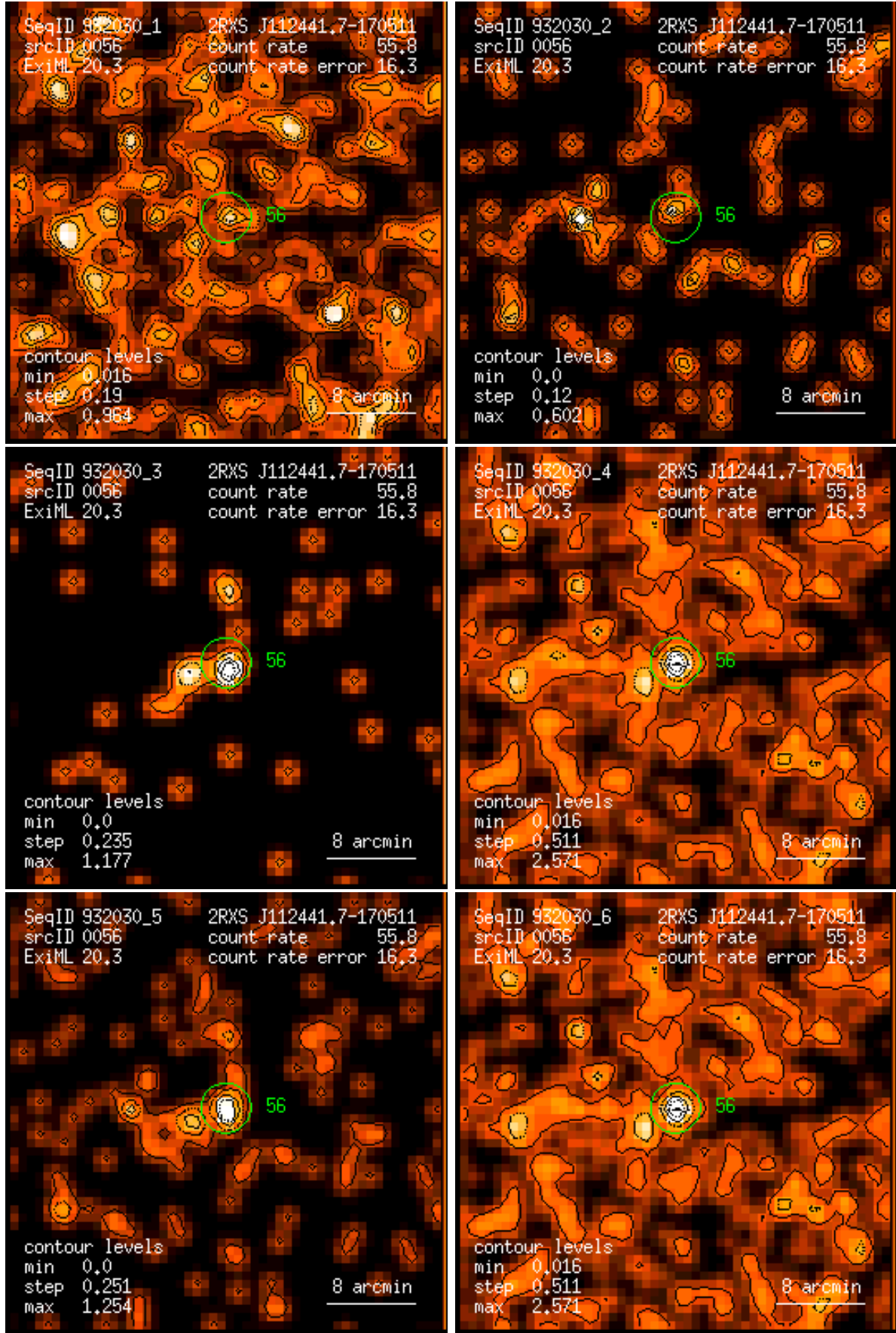
Figure 56: RASS 932030: detection 0056: band rate images, Gaussian filter: (1) PSPC channels 11 – 41, (2) 52 – 90, (3) 91 – 201, (4) 11 – 235, (5) 52 – 201, (6) 11 – 201. Broad band rates in counts/ks. Band rate contour levels in counts/ks/arcmin 2 .
