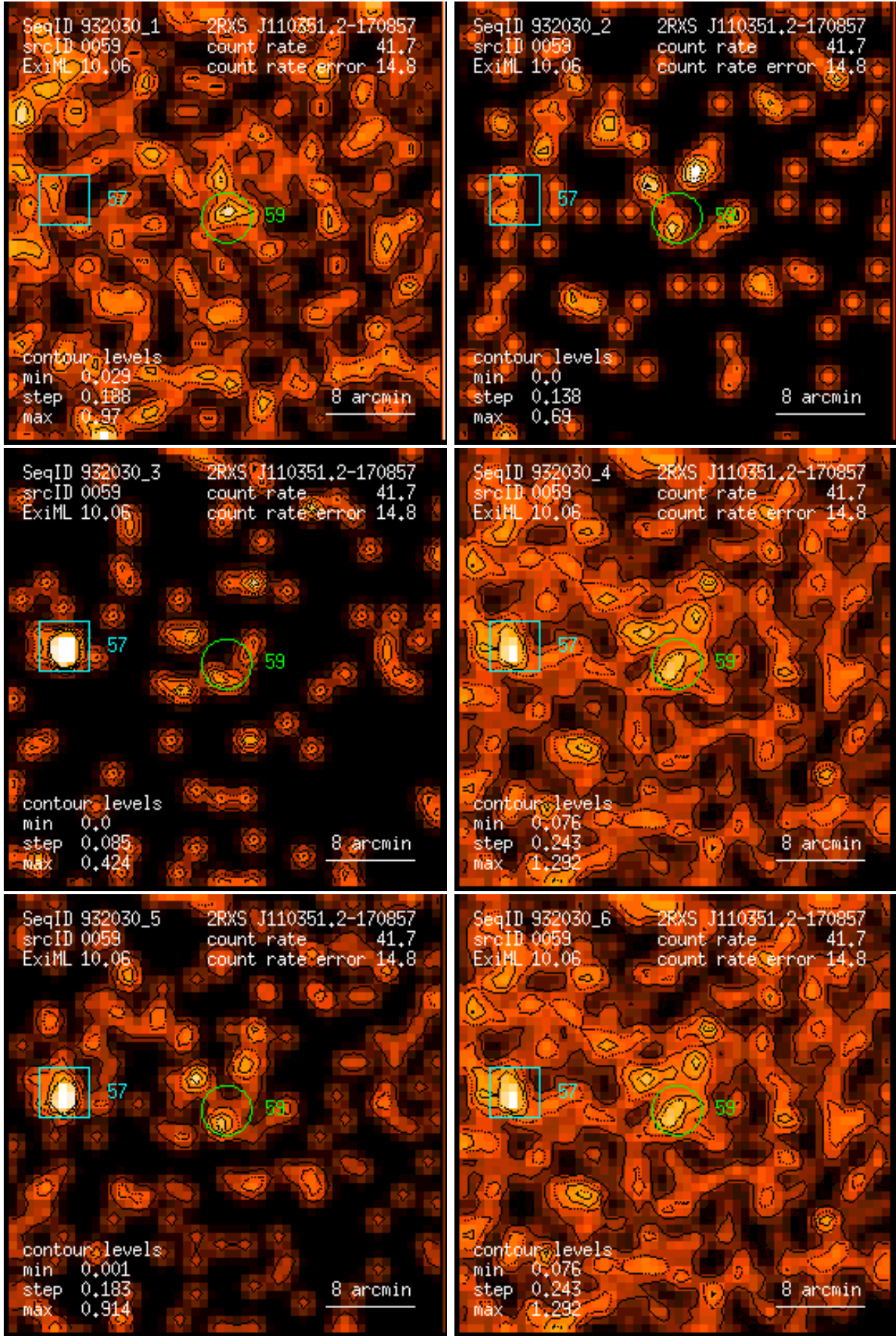
Figure 59: RASS 932030: detection 0059: band rate images, Gaussian filter: (1) PSPC channels 11 – 41, (2) 52 – 90, (3) 91 – 201, (4) 11 – 235, (5) 52 – 201, (6) 11 – 201. Broad band rates in counts/ks. Band rate contour levels in counts/ks/arcmin 2 .
