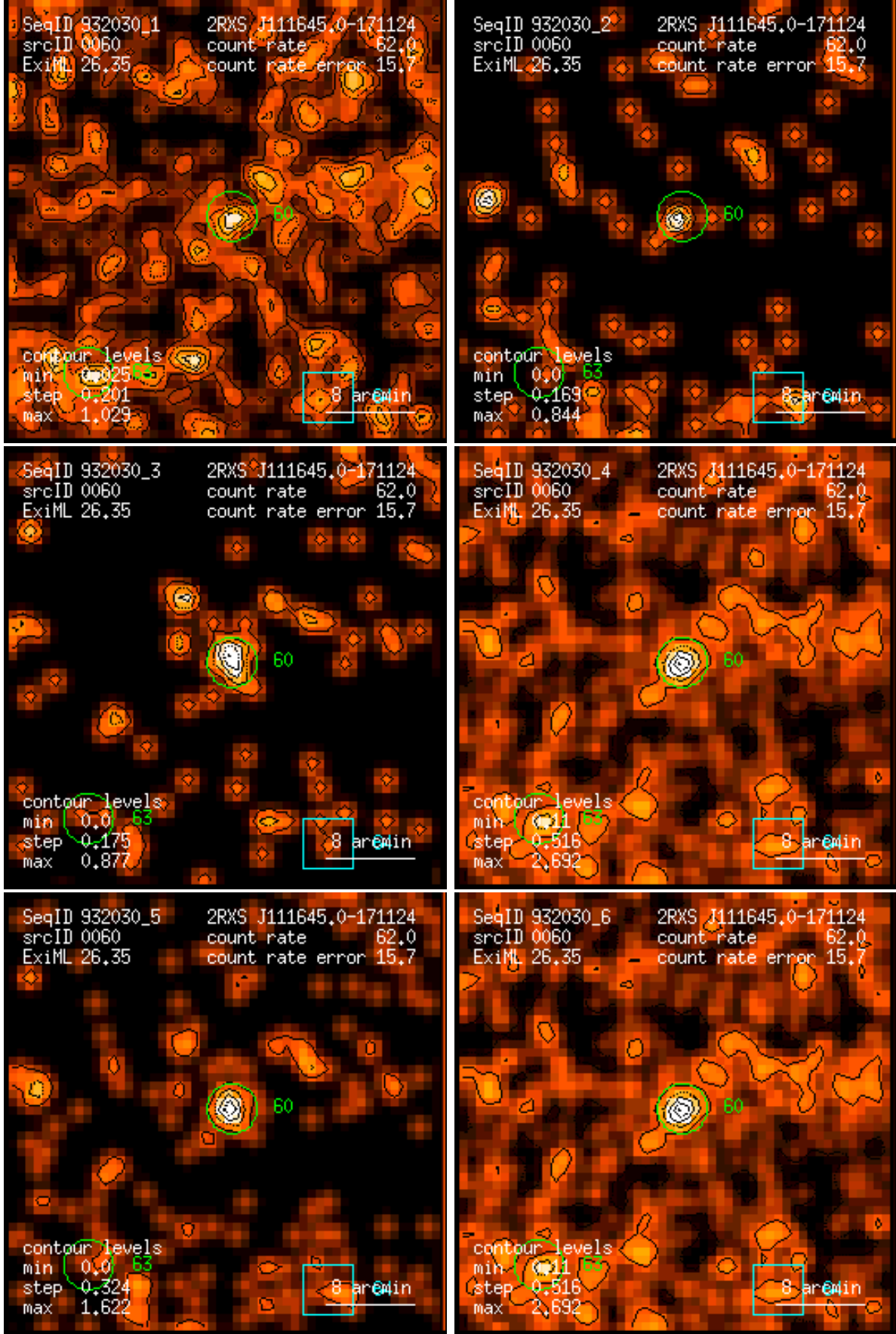
Figure 60: RASS 932030: detection 0060: band rate images, Gaussian filter: (1) PSPC channels 11 – 41, (2) 52 – 90, (3) 91 – 201, (4) 11 – 235, (5) 52 – 201, (6) 11 – 201. Broad band rates in counts/ks. Band rate contour levels in counts/ks/arcmin 2 .
