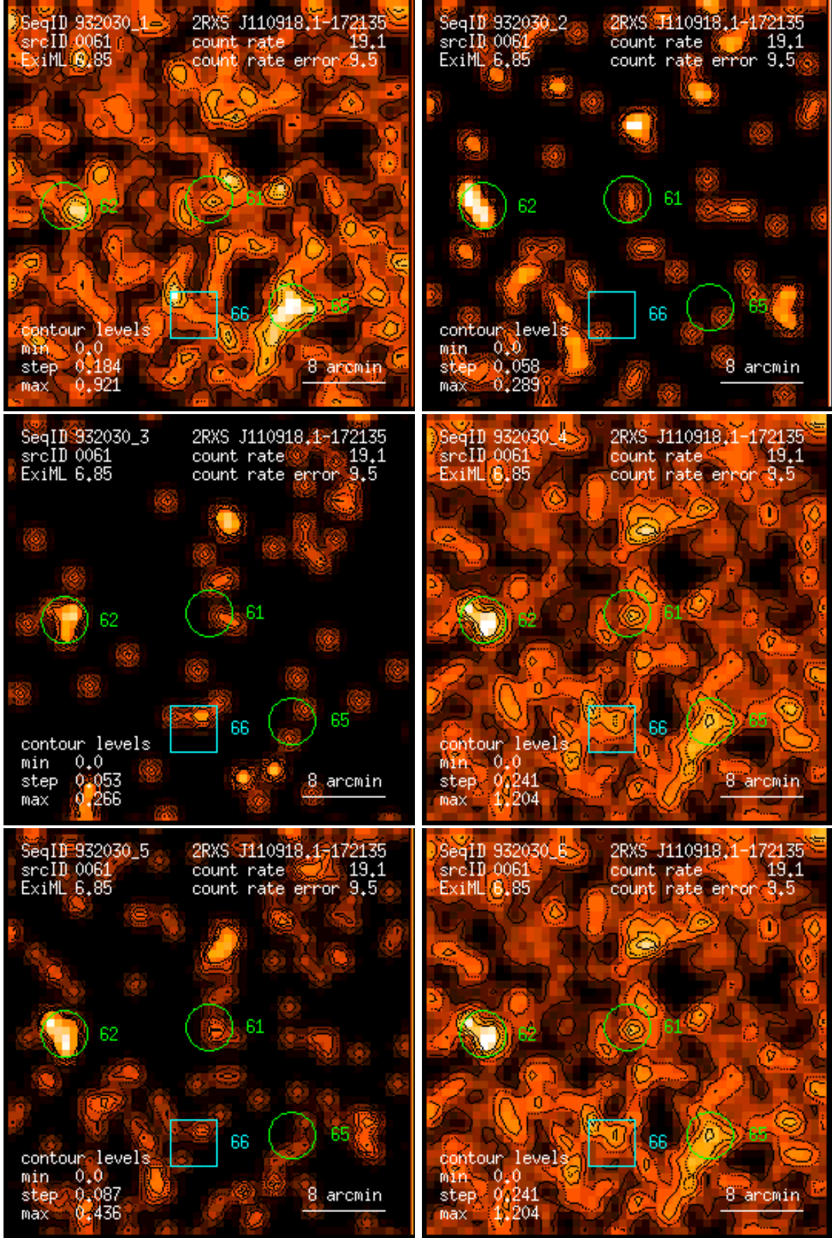
Figure 61: RASS 932030: detection 0061: band rate images, Gaussian filter: (1) PSPC channels 11 – 41, (2) 52 – 90, (3) 91 – 201, (4) 11 – 235, (5) 52 – 201, (6) 11 – 201. Broad band rates in counts/ks. Band rate contour levels in counts/ks/arcmin 2 .
