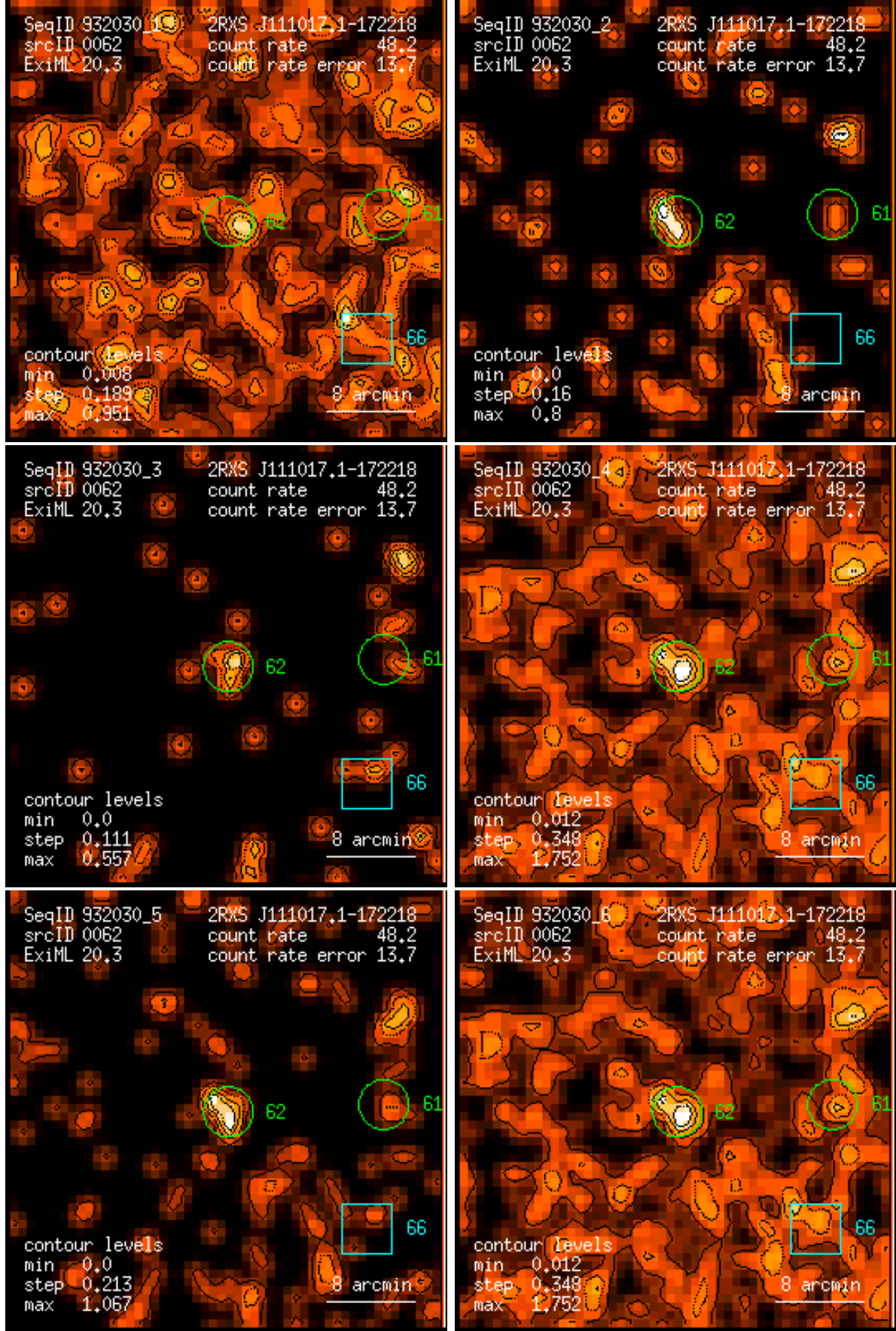
Figure 62: RASS 932030: detection 0062: band rate images, Gaussian filter: (1) PSPC channels 11 – 41, (2) 52 – 90, (3) 91 – 201, (4) 11 – 235, (5) 52 – 201, (6) 11 – 201. Broad band rates in counts/ks. Band rate contour levels in counts/ks/arcmin 2 .
