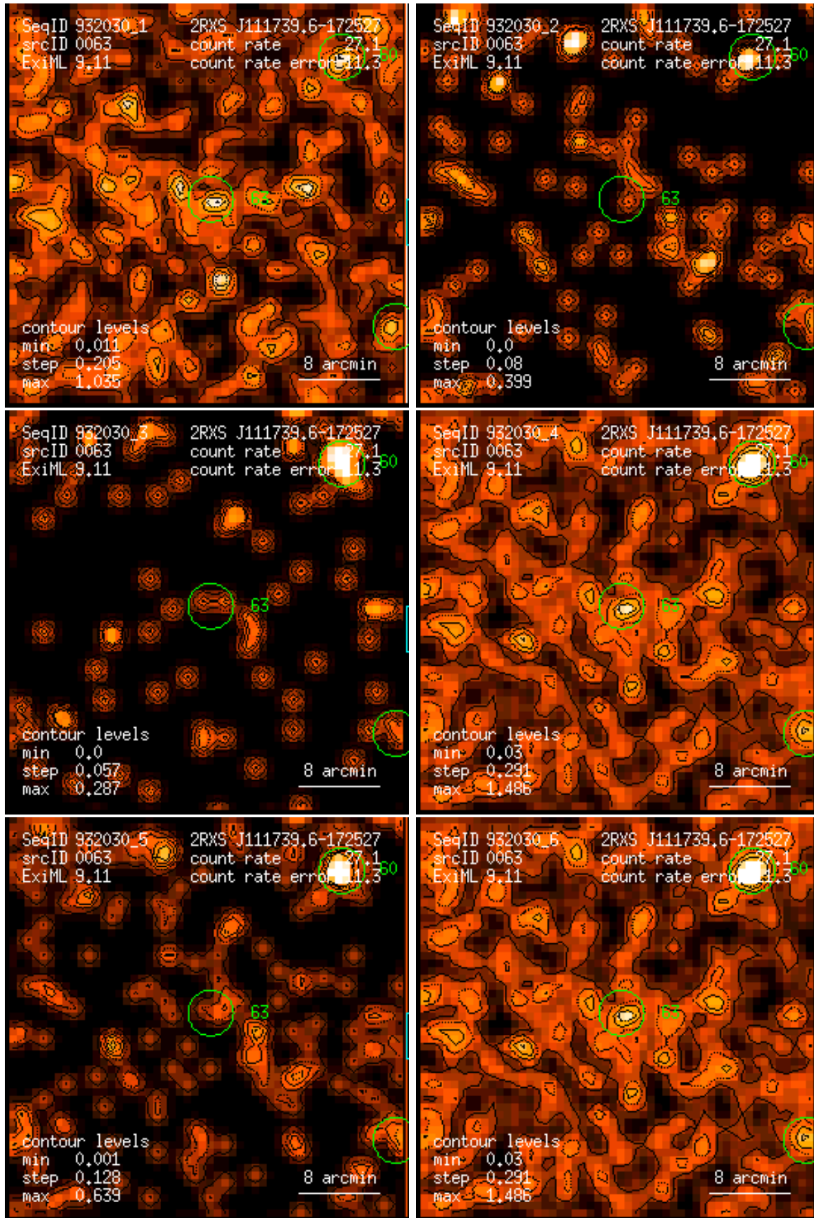
Figure 63: RASS 932030: detection 0063: band rate images, Gaussian filter: (1) PSPC channels 11 – 41, (2) 52 – 90, (3) 91 – 201, (4) 11 – 235, (5) 52 – 201, (6) 11 – 201. Broad band rates in counts/ks. Band rate contour levels in counts/ks/arcmin 2 .
