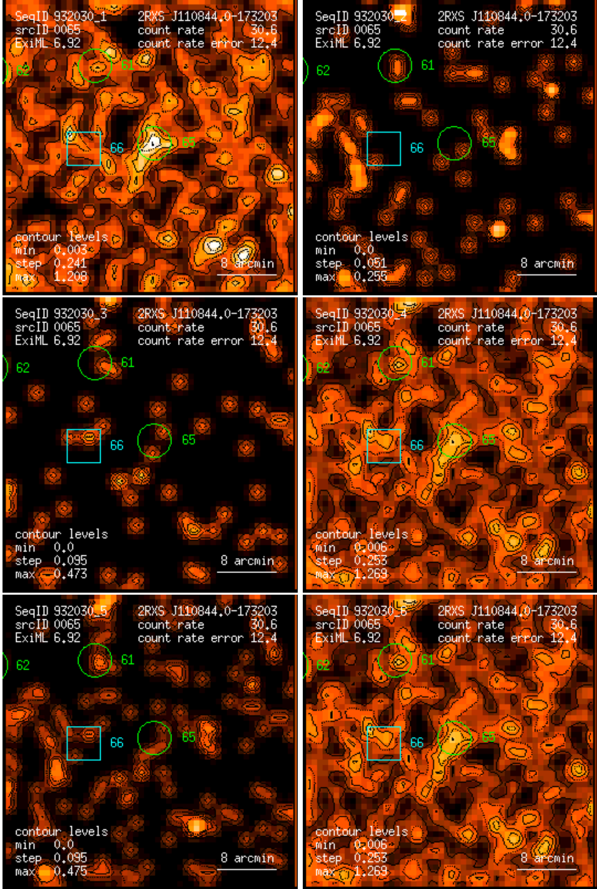
Figure 65: RASS 932030: detection 0065: band rate images, Gaussian filter: (1) PSPC channels 11 – 41, (2) 52 – 90, (3) 91 – 201, (4) 11 – 235, (5) 52 – 201, (6) 11 – 201. Broad band rates in counts/ks. Band rate contour levels in counts/ks/arcmin 2 .
