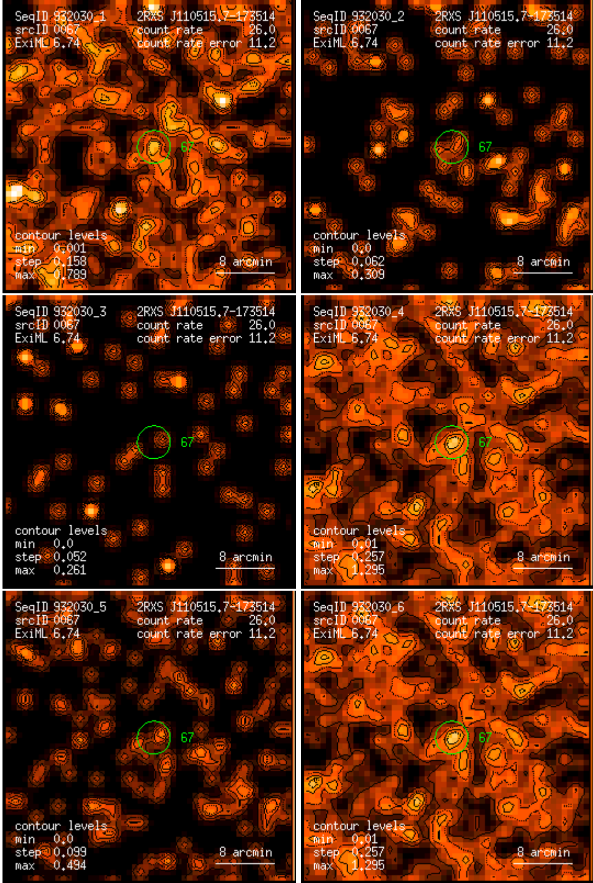
Figure 67: RASS 932030: detection 0067: band rate images, Gaussian filter: (1) PSPC channels 11 – 41, (2) 52 – 90, (3) 91 – 201, (4) 11 – 235, (5) 52 – 201, (6) 11 – 201. Broad band rates in counts/ks. Band rate contour levels in counts/ks/arcmin 2 .
