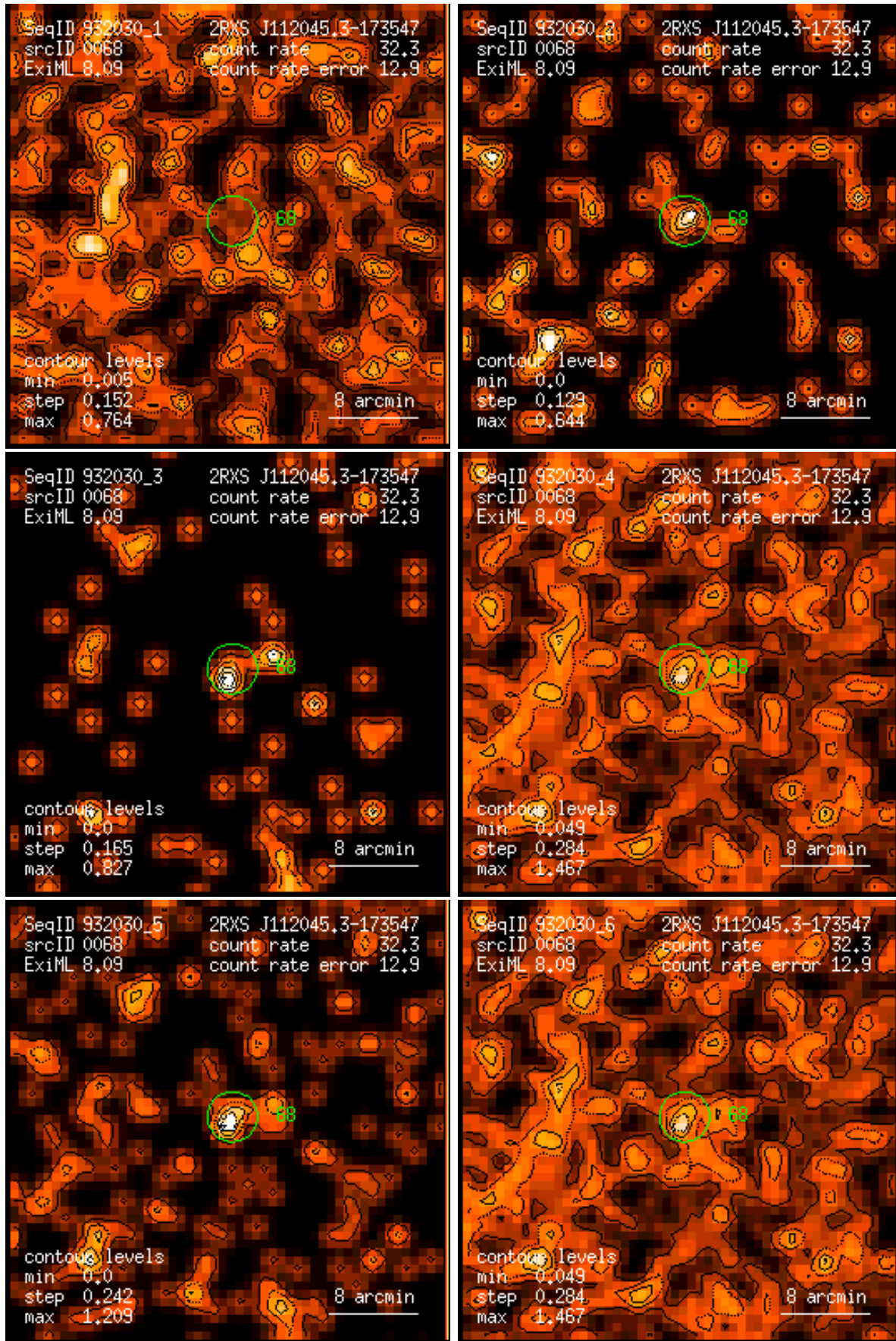
Figure 68: RASS 932030: detection 0068: band rate images, Gaussian filter: (1) PSPC channels 11 – 41, (2) 52 – 90, (3) 91 – 201, (4) 11 – 235, (5) 52 – 201, (6) 11 – 201. Broad band rates in counts/ks. Band rate contour levels in counts/ks/arcmin 2 .
