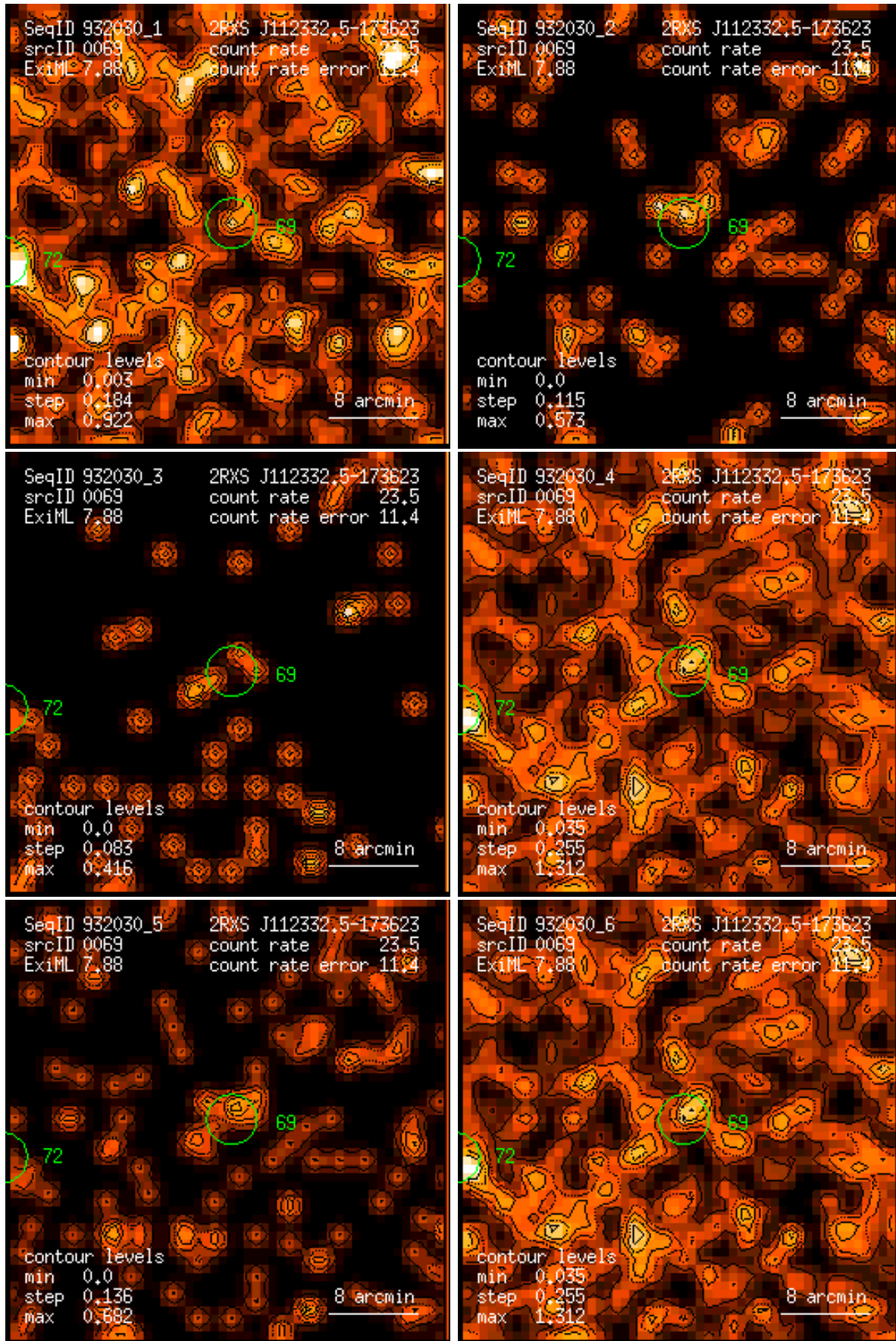
Figure 69: RASS 932030: detection 0069: band rate images, Gaussian filter: (1) PSPC channels 11 – 41, (2) 52 – 90, (3) 91 – 201, (4) 11 – 235, (5) 52 – 201, (6) 11 – 201. Broad band rates in counts/ks. Band rate contour levels in counts/ks/arcmin 2 .
