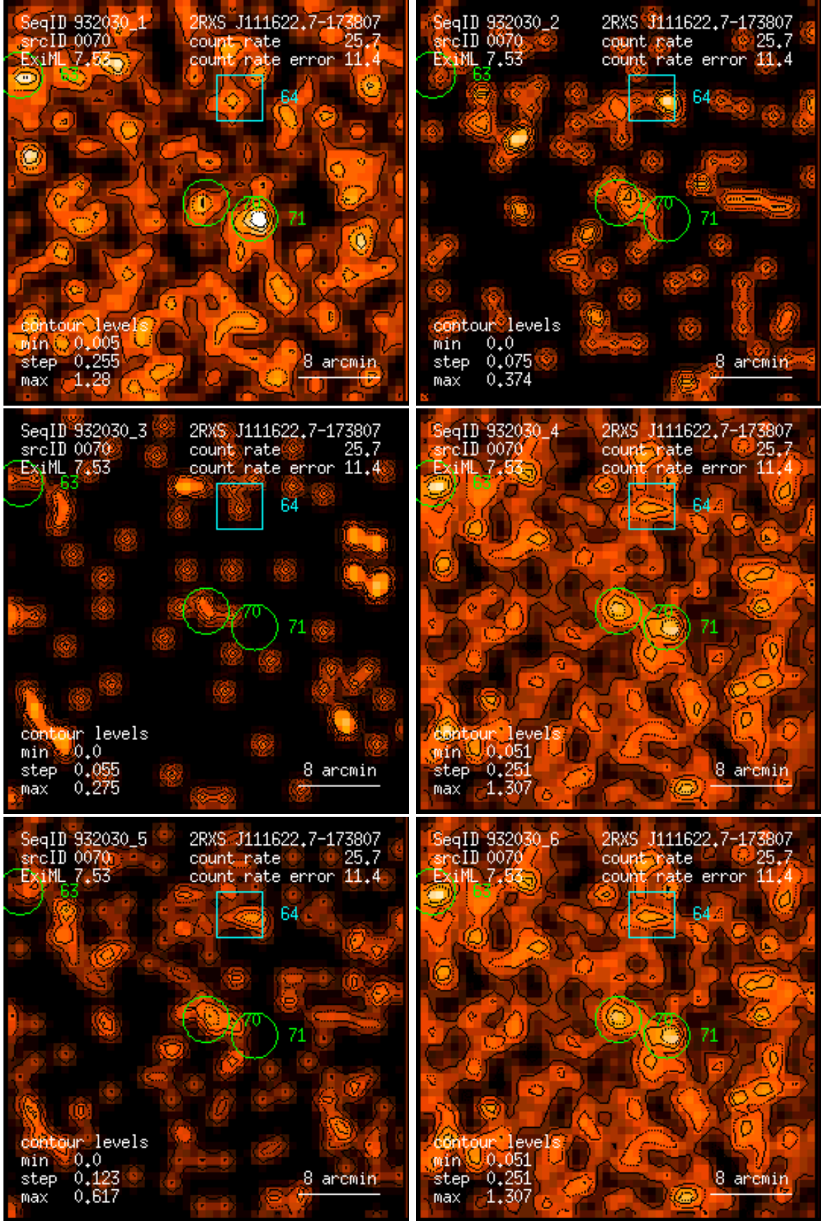
Figure 70: RASS 932030: detection 0070: band rate images, Gaussian filter: (1) PSPC channels 11 – 41, (2) 52 – 90, (3) 91 – 201, (4) 11 – 235, (5) 52 – 201, (6) 11 – 201. Broad band rates in counts/ks. Band rate contour levels in counts/ks/arcmin 2 .
