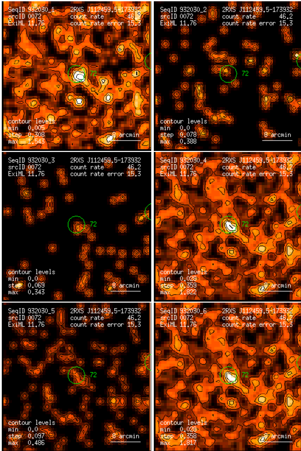
Figure 72: RASS 932030: detection 0072: band rate images, Gaussian filter: (1) PSPC channels 11 – 41, (2) 52 – 90, (3) 91 – 201, (4) 11 – 235, (5) 52 – 201, (6) 11 – 201. Broad band rates in counts/ks. Band rate contour levels in counts/ks/arcmin 2 .
