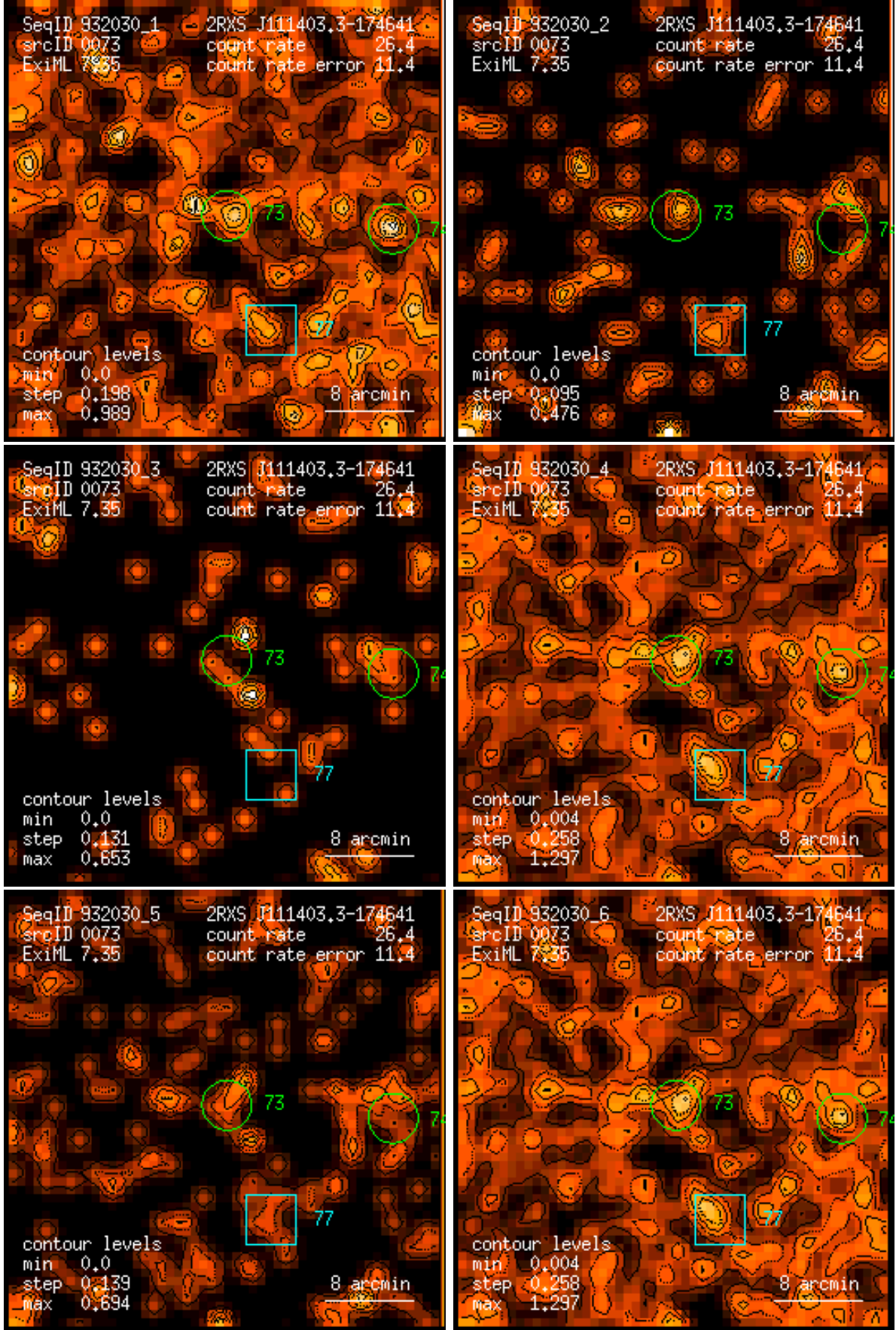
Figure 73: RASS 932030: detection 0073: band rate images, Gaussian filter: (1) PSPC channels 11 – 41, (2) 52 – 90, (3) 91 – 201, (4) 11 – 235, (5) 52 – 201, (6) 11 – 201. Broad band rates in counts/ks. Band rate contour levels in counts/ks/arcmin 2 .
