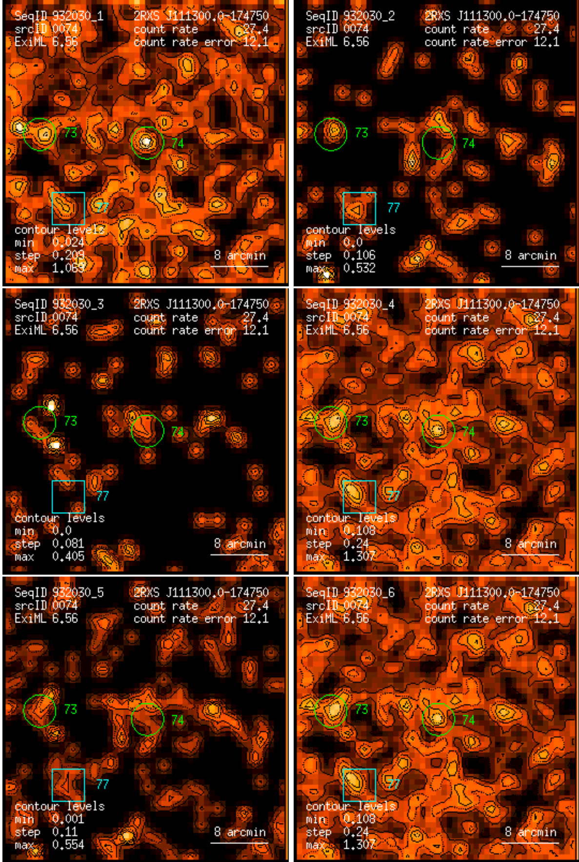
Figure 74: RASS 932030: detection 0074: band rate images, Gaussian filter: (1) PSPC channels 11 – 41, (2) 52 – 90, (3) 91 – 201, (4) 11 – 235, (5) 52 – 201, (6) 11 – 201. Broad band rates in counts/ks. Band rate contour levels in counts/ks/arcmin 2 .
