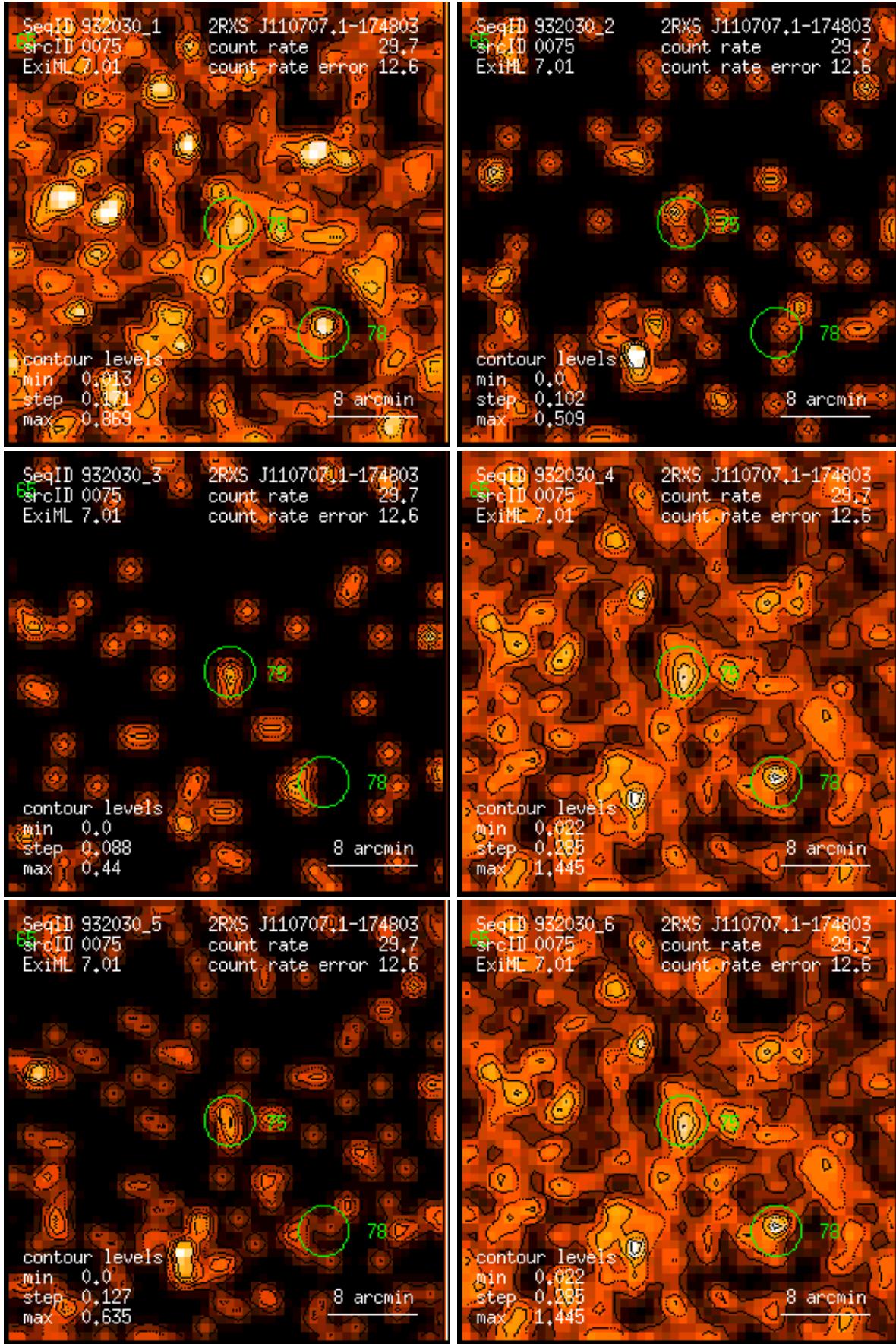
Figure 75: RASS 932030: detection 0075: band rate images, Gaussian filter: (1) PSPC channels 11 – 41, (2) 52 – 90, (3) 91 – 201, (4) 11 – 235, (5) 52 – 201, (6) 11 – 201. Broad band rates in counts/ks. Band rate contour levels in counts/ks/arcmin 2 .
