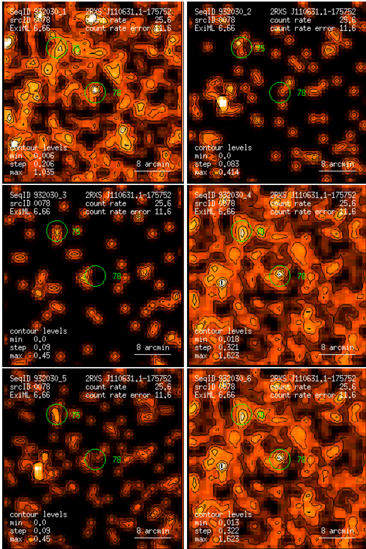
Figure 78: RASS 932030: detection 0078: band rate images, Gaussian filter: (1) PSPC channels 11 – 41, (2) 52 – 90, (3) 91 – 201, (4) 11 – 235, (5) 52 – 201, (6) 11 – 201. Broad band rates in counts/ks. Band rate contour levels in counts/ks/arcmin 2 .
