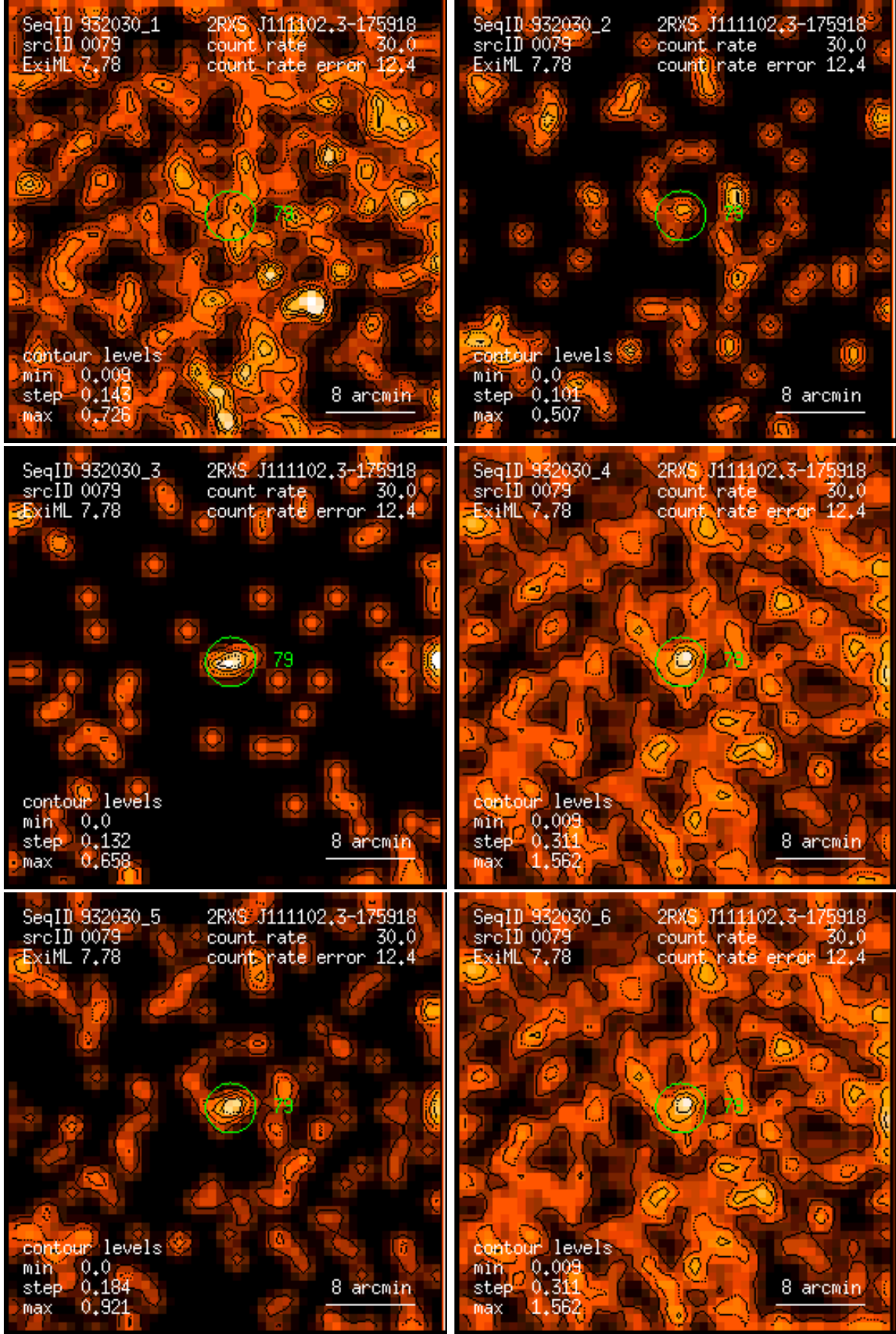
Figure 79: RASS 932030: detection 0079: band rate images, Gaussian filter: (1) PSPC channels 11 – 41, (2) 52 – 90, (3) 91 – 201, (4) 11 – 235, (5) 52 – 201, (6) 11 – 201. Broad band rates in counts/ks. Band rate contour levels in counts/ks/arcmin 2 .
