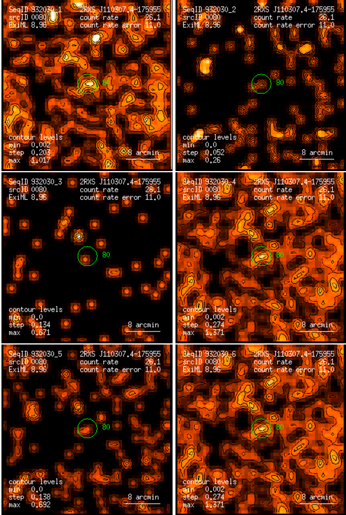
Figure 80: RASS 932030: detection 0080: band rate images, Gaussian filter: (1) PSPC channels 11 – 41, (2) 52 – 90, (3) 91 – 201, (4) 11 – 235, (5) 52 – 201, (6) 11 – 201. Broad band rates in counts/ks. Band rate contour levels in counts/ks/arcmin 2 .
