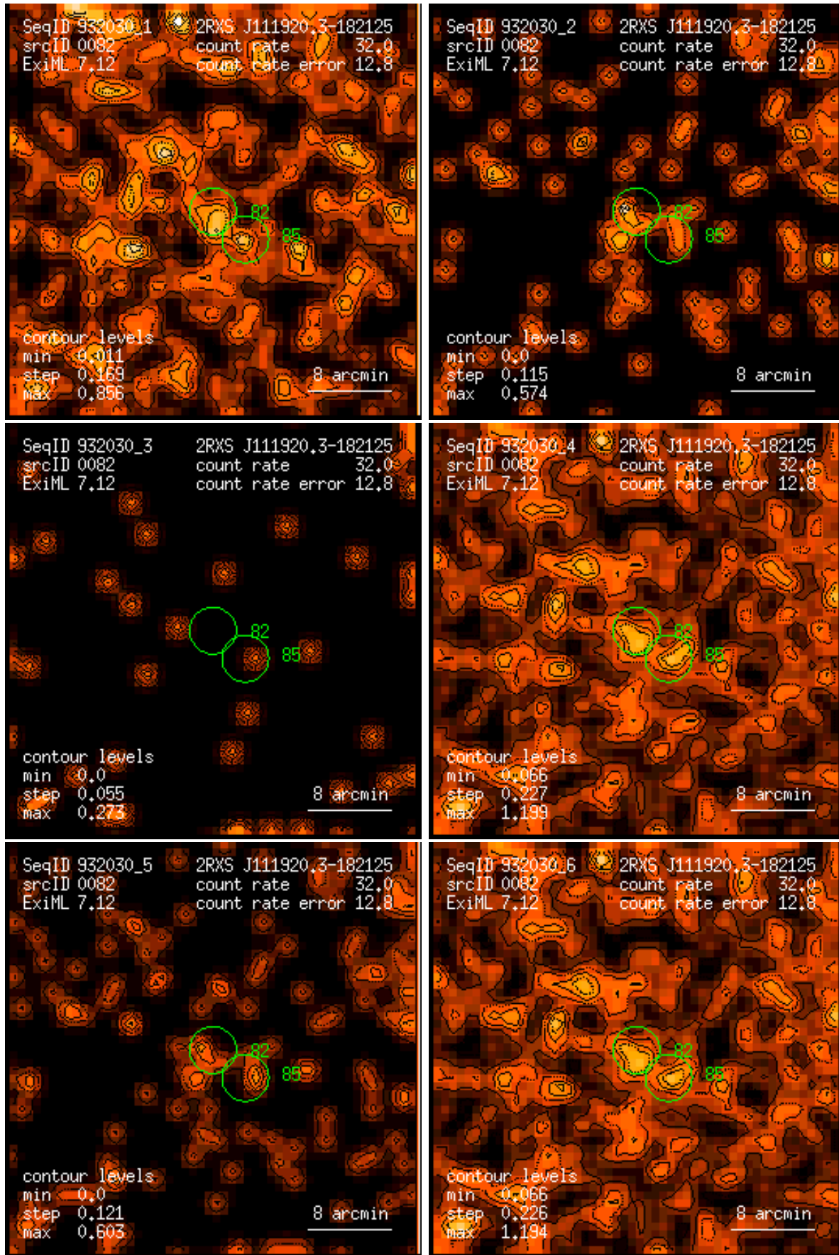
Figure 82: RASS 932030: detection 0082: band rate images, Gaussian filter: (1) PSPC channels 11 – 41, (2) 52 – 90, (3) 91 – 201, (4) 11 – 235, (5) 52 – 201, (6) 11 – 201. Broad band rates in counts/ks. Band rate contour levels in counts/ks/arcmin 2 .
