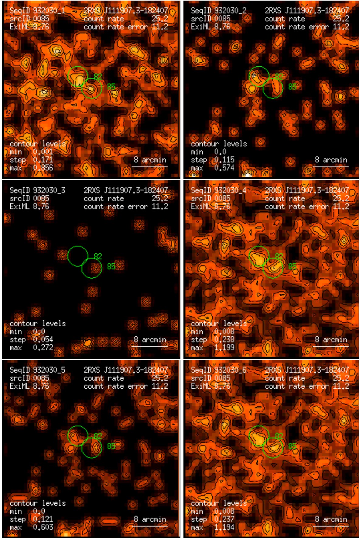
Figure 85: RASS 932030: detection 0085: band rate images, Gaussian filter: (1) PSPC channels 11 – 41, (2) 52 – 90, (3) 91 – 201, (4) 11 – 235, (5) 52 – 201, (6) 11 – 201. Broad band rates in counts/ks. Band rate contour levels in counts/ks/arcmin 2 .
