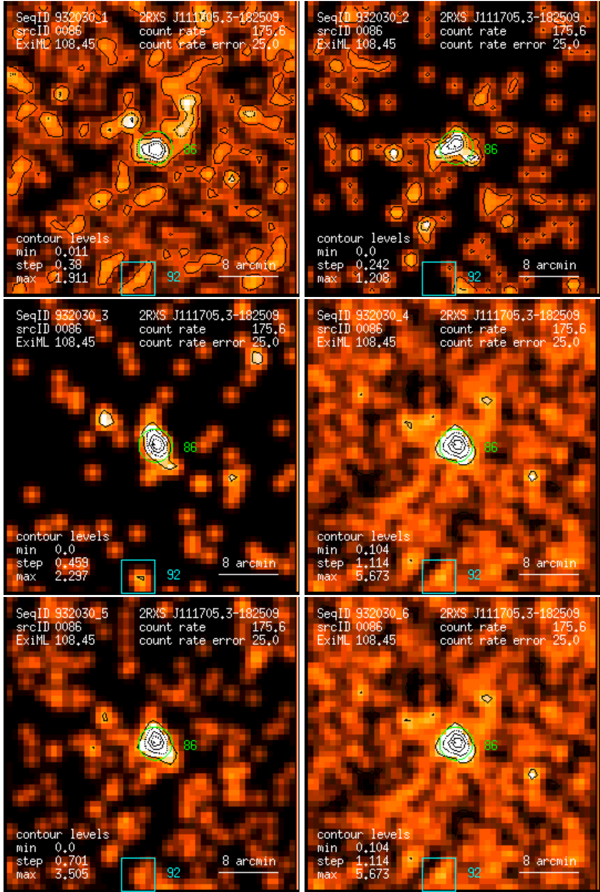
Figure 86: RASS 932030: detection 0086: band rate images, Gaussian filter: (1) PSPC channels 11 – 41, (2) 52 – 90, (3) 91 – 201, (4) 11 – 235, (5) 52 – 201, (6) 11 – 201. Broad band rates in counts/ks. Band rate contour levels in counts/ks/arcmin 2 .
