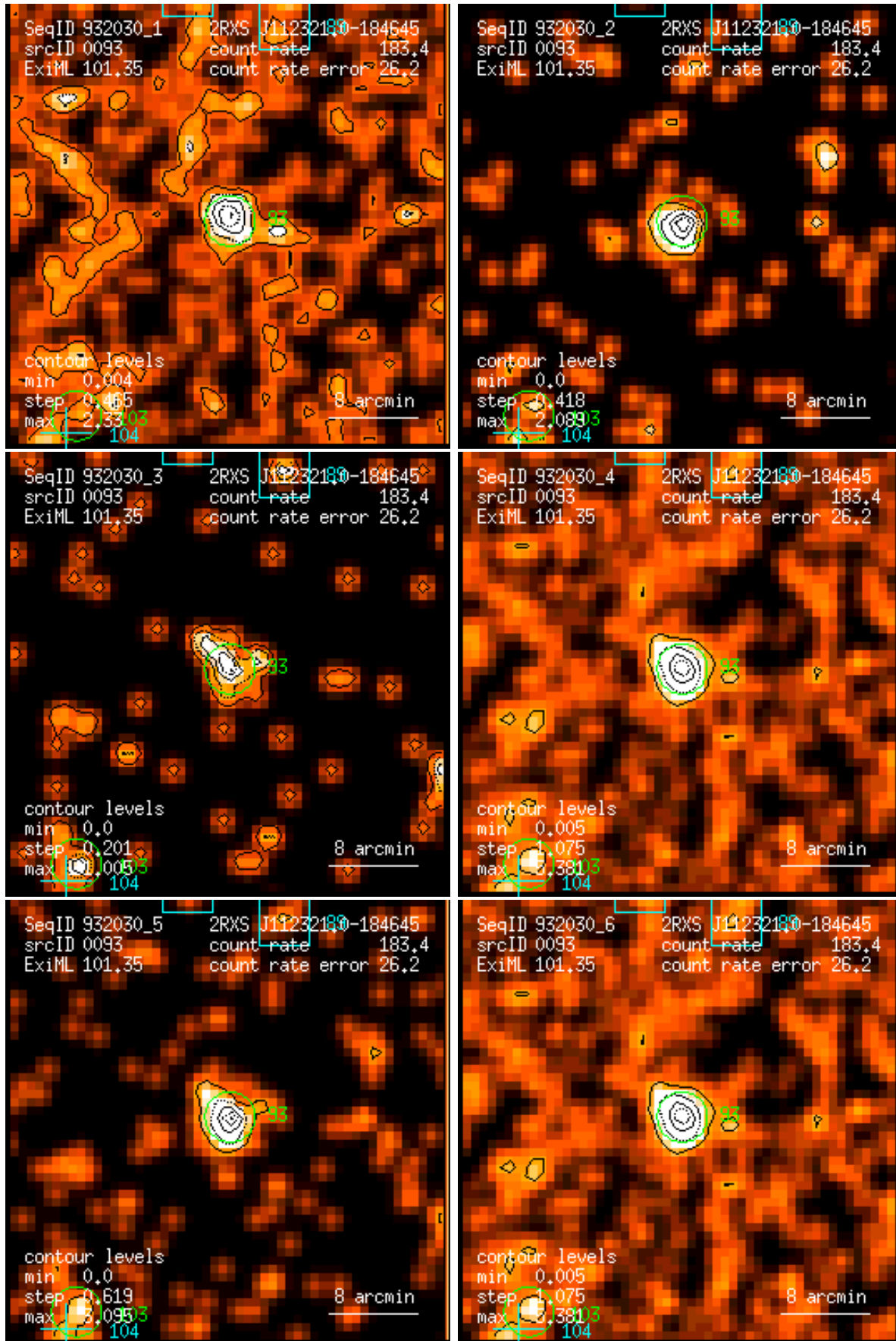
Figure 93: RASS 932030: detection 0093: band rate images, Gaussian filter: (1) PSPC channels 11 – 41, (2) 52 – 90, (3) 91 – 201, (4) 11 – 235, (5) 52 – 201, (6) 11 – 201. Broad band rates in counts/ks. Band rate contour levels in counts/ks/arcmin 2 .
