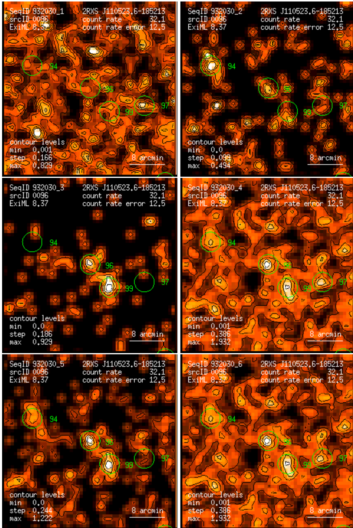
Figure 96: RASS 932030: detection 0096: band rate images, Gaussian filter: (1) PSPC channels 11 – 41, (2) 52 – 90, (3) 91 – 201, (4) 11 – 235, (5) 52 – 201, (6) 11 – 201. Broad band rates in counts/ks. Band rate contour levels in counts/ks/arcmin 2 .
