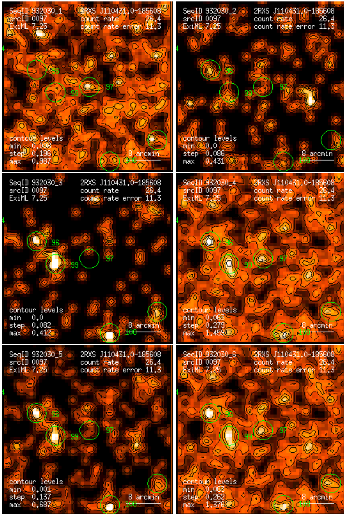
Figure 97: RASS 932030: detection 0097: band rate images, Gaussian filter: (1) PSPC channels 11 – 41, (2) 52 – 90, (3) 91 – 201, (4) 11 – 235, (5) 52 – 201, (6) 11 – 201. Broad band rates in counts/ks. Band rate contour levels in counts/ks/arcmin 2 .
