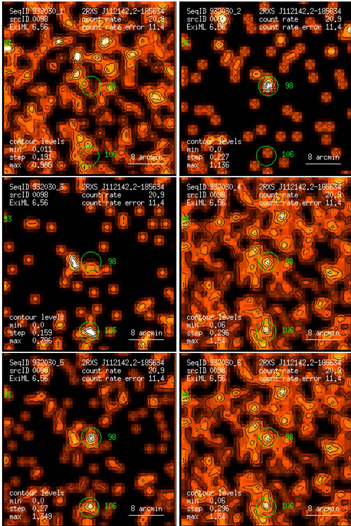
Figure 98: RASS 932030: detection 0098: band rate images, Gaussian filter: (1) PSPC channels 11 – 41, (2) 52 – 90, (3) 91 – 201, (4) 11 – 235, (5) 52 – 201, (6) 11 – 201. Broad band rates in counts/ks. Band rate contour levels in counts/ks/arcmin 2 .
