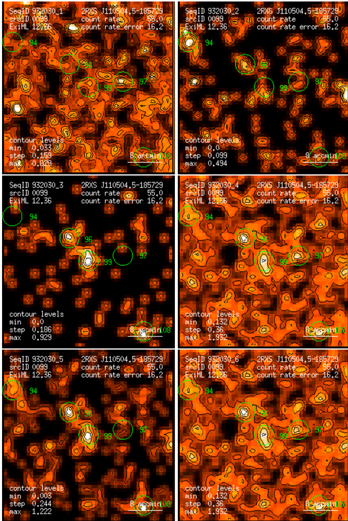
Figure 99: RASS 932030: detection 0099: band rate images, Gaussian filter: (1) PSPC channels 11 – 41, (2) 52 – 90, (3) 91 – 201, (4) 11 – 235, (5) 52 – 201, (6) 11 – 201. Broad band rates in counts/ks. Band rate contour levels in counts/ks/arcmin 2 .
