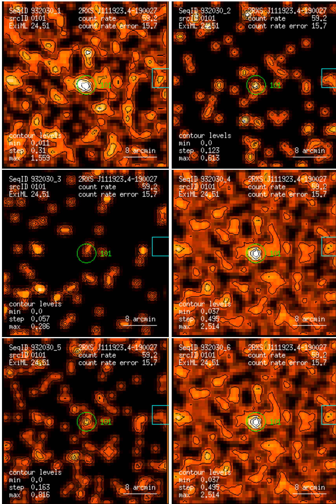
Figure 101: RASS 932030: detection 0101: band rate images, Gaussian filter: (1) PSPC channels 11 – 41, (2) 52 – 90, (3) 91 – 201, (4) 11 – 235, (5) 52 – 201, (6) 11 – 201. Broad band rates in counts/ks. Band rate contour levels in counts/ks/arcmin 2 .
