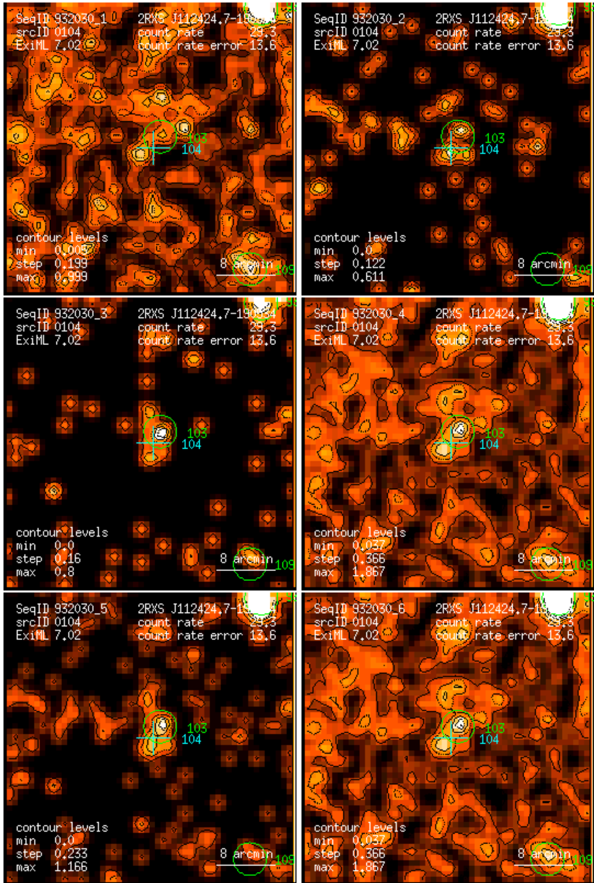
Figure 104: RASS 932030: detection 0104: band rate images, Gaussian filter: (1) PSPC channels 11 – 41, (2) 52 – 90, (3) 91 – 201, (4) 11 – 235, (5) 52 – 201, (6) 11 – 201. Broad band rates in counts/ks. Band rate contour levels in counts/ks/arcmin 2 .
