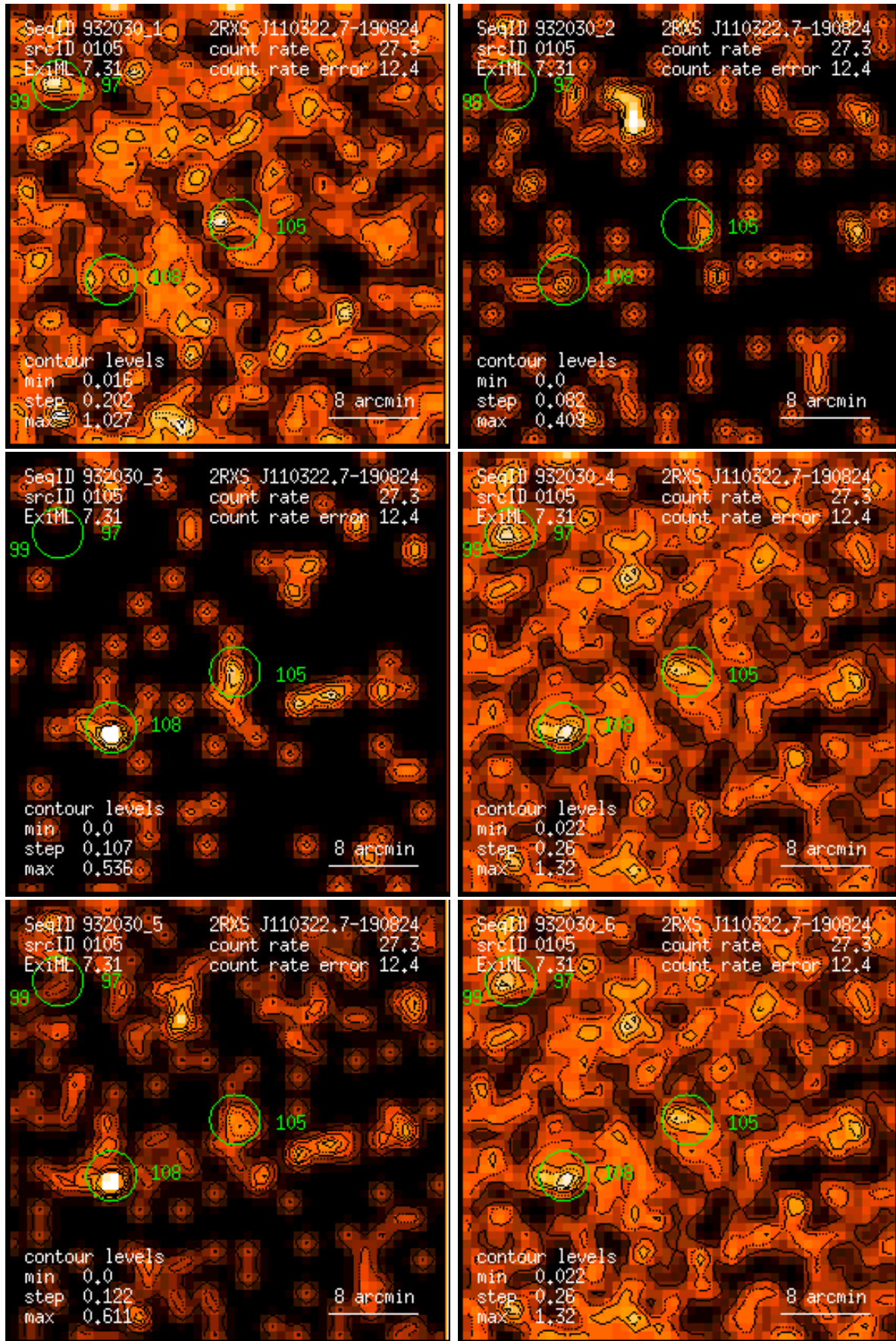
Figure 105: RASS 932030: detection 0105: band rate images, Gaussian filter: (1) PSPC channels 11 – 41, (2) 52 – 90, (3) 91 – 201, (4) 11 – 235, (5) 52 – 201, (6) 11 – 201. Broad band rates in counts/ks. Band rate contour levels in counts/ks/arcmin 2 .
