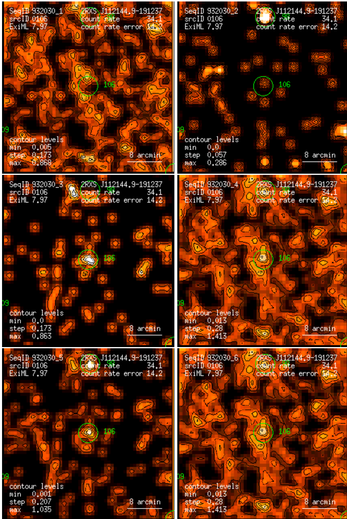
Figure 106: RASS 932030: detection 0106: band rate images, Gaussian filter: (1) PSPC channels 11 – 41, (2) 52 – 90, (3) 91 – 201, (4) 11 – 235, (5) 52 – 201, (6) 11 – 201. Broad band rates in counts/ks. Band rate contour levels in counts/ks/arcmin 2 .
