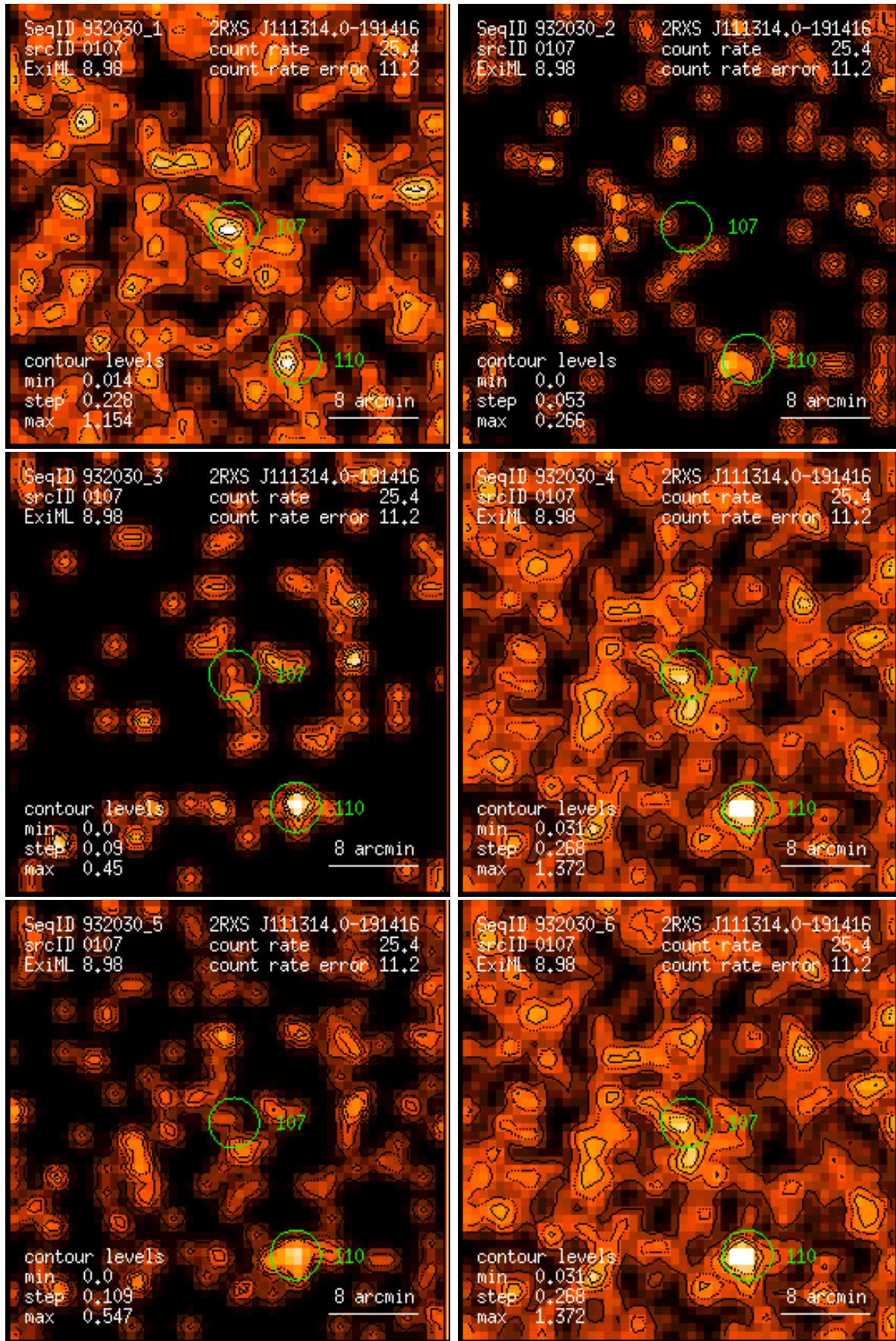
Figure 107: RASS 932030: detection 0107: band rate images, Gaussian filter: (1) PSPC channels 11 – 41, (2) 52 – 90, (3) 91 – 201, (4) 11 – 235, (5) 52 – 201, (6) 11 – 201. Broad band rates in counts/ks. Band rate contour levels in counts/ks/arcmin 2 .
