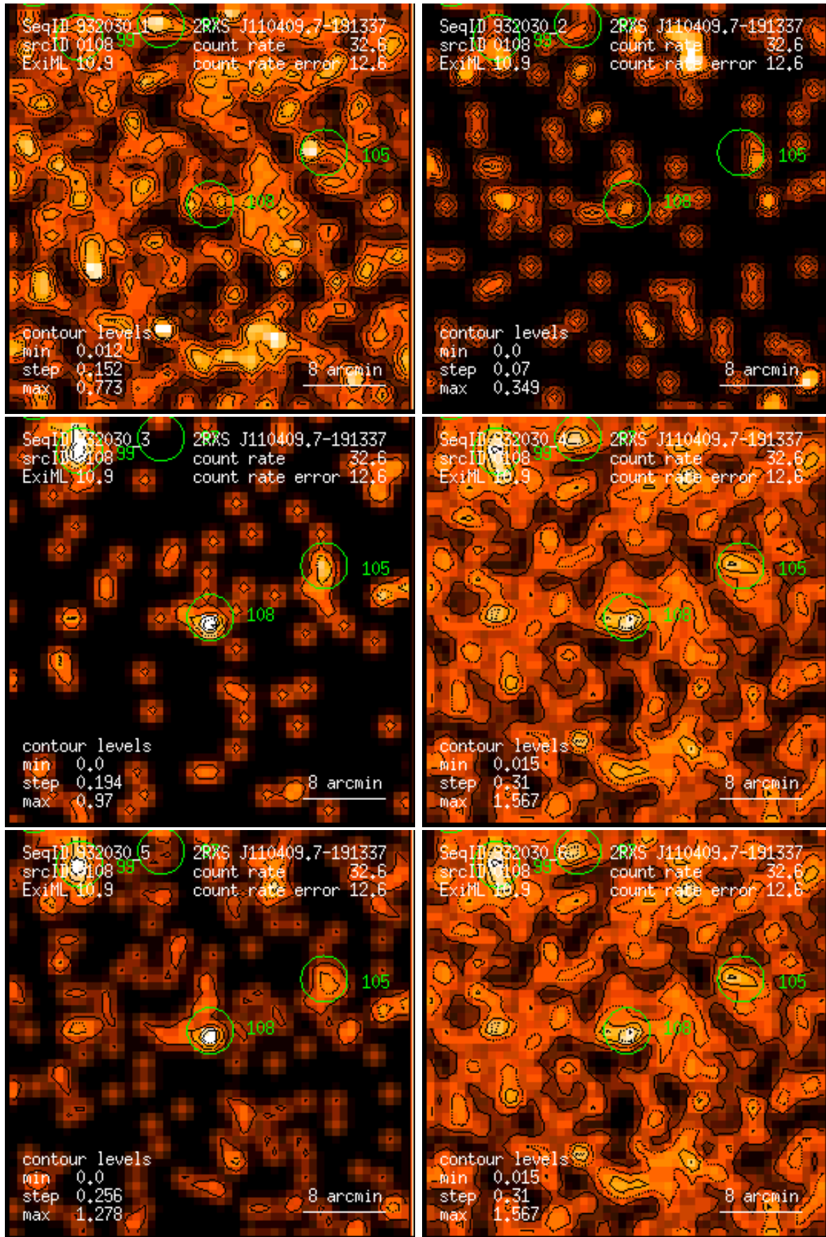
Figure 108: RASS 932030: detection 0108: band rate images, Gaussian filter: (1) PSPC channels 11 – 41, (2) 52 – 90, (3) 91 – 201, (4) 11 – 235, (5) 52 – 201, (6) 11 – 201. Broad band rates in counts/ks. Band rate contour levels in counts/ks/arcmin 2 .
