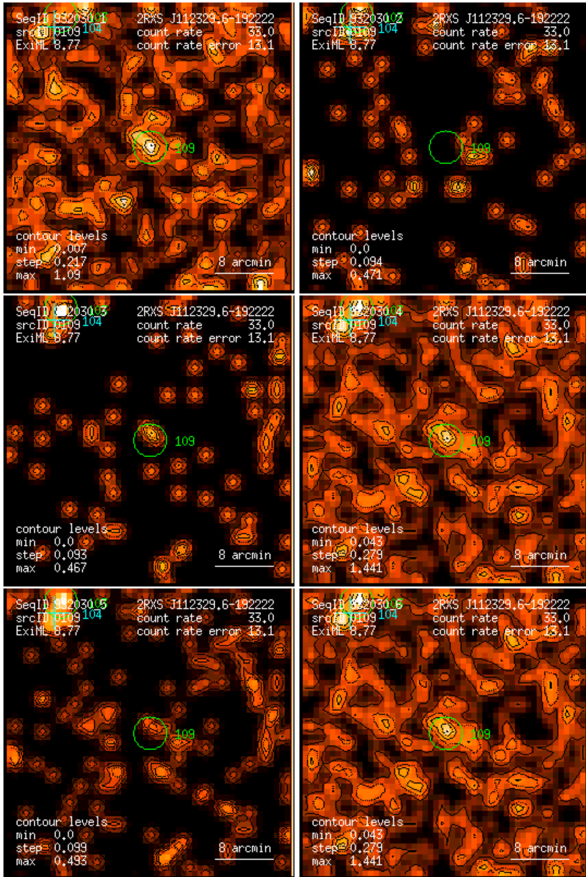
Figure 109: RASS 932030: detection 0109: band rate images, Gaussian filter: (1) PSPC channels 11 – 41, (2) 52 – 90, (3) 91 – 201, (4) 11 – 235, (5) 52 – 201, (6) 11 – 201. Broad band rates in counts/ks. Band rate contour levels in counts/ks/arcmin 2 .
