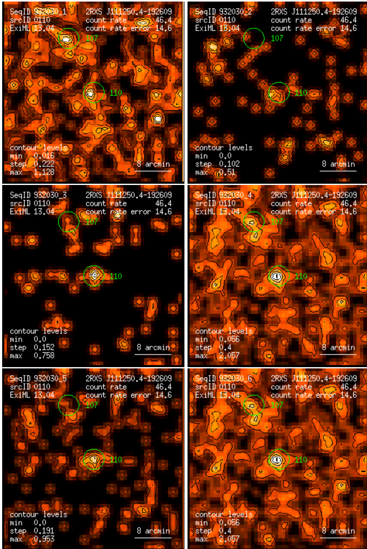
Figure 110: RASS 932030: detection 0110: band rate images, Gaussian filter: (1) PSPC channels 11 – 41, (2) 52 – 90, (3) 91 – 201, (4) 11 – 235, (5) 52 – 201, (6) 11 – 201. Broad band rates in counts/ks. Band rate contour levels in counts/ks/arcmin 2 .
